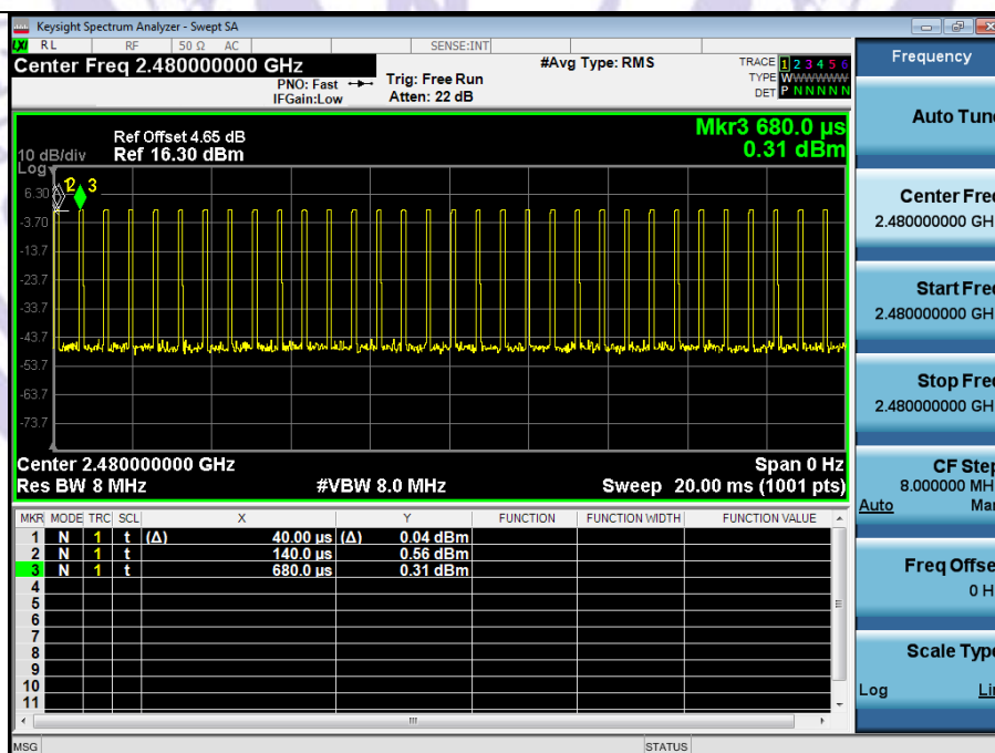
Duty Cycle_NVNT_ANT1_1Mbps_2480
