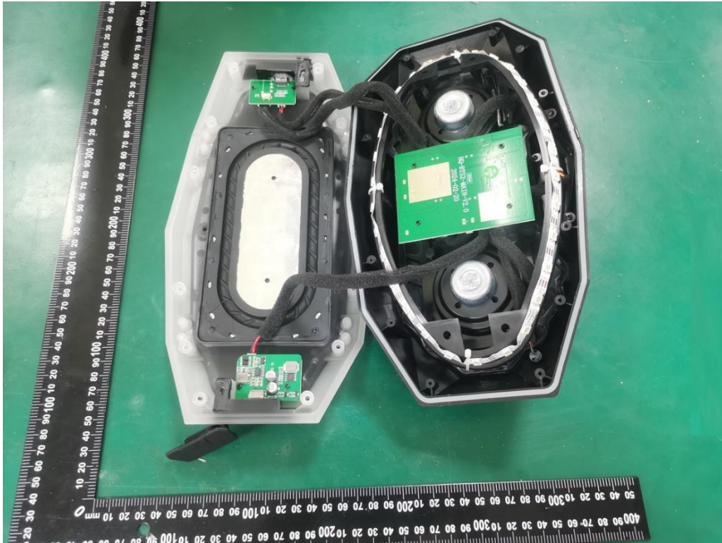
Internal Photo FCC ID: 2BD87-OT4803
