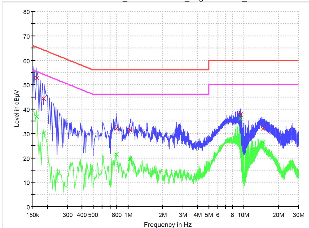
Plots No. 24: AC Mains Conducted Emission _ AC 120V/60Hz _ High Channel _ Line
