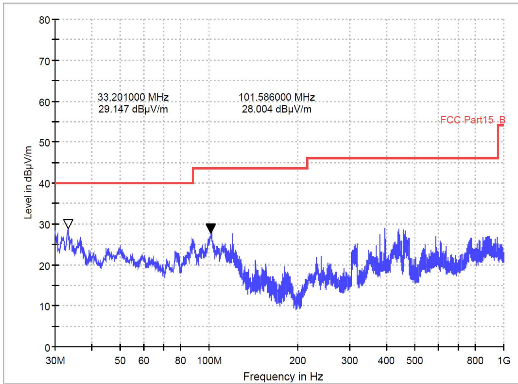
Plots No. 1: 30 MHz to 1 GHz, Horizontal / Vertical Polarization _ High Channel
