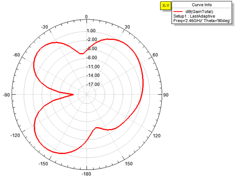
Radiation Pattern 2
