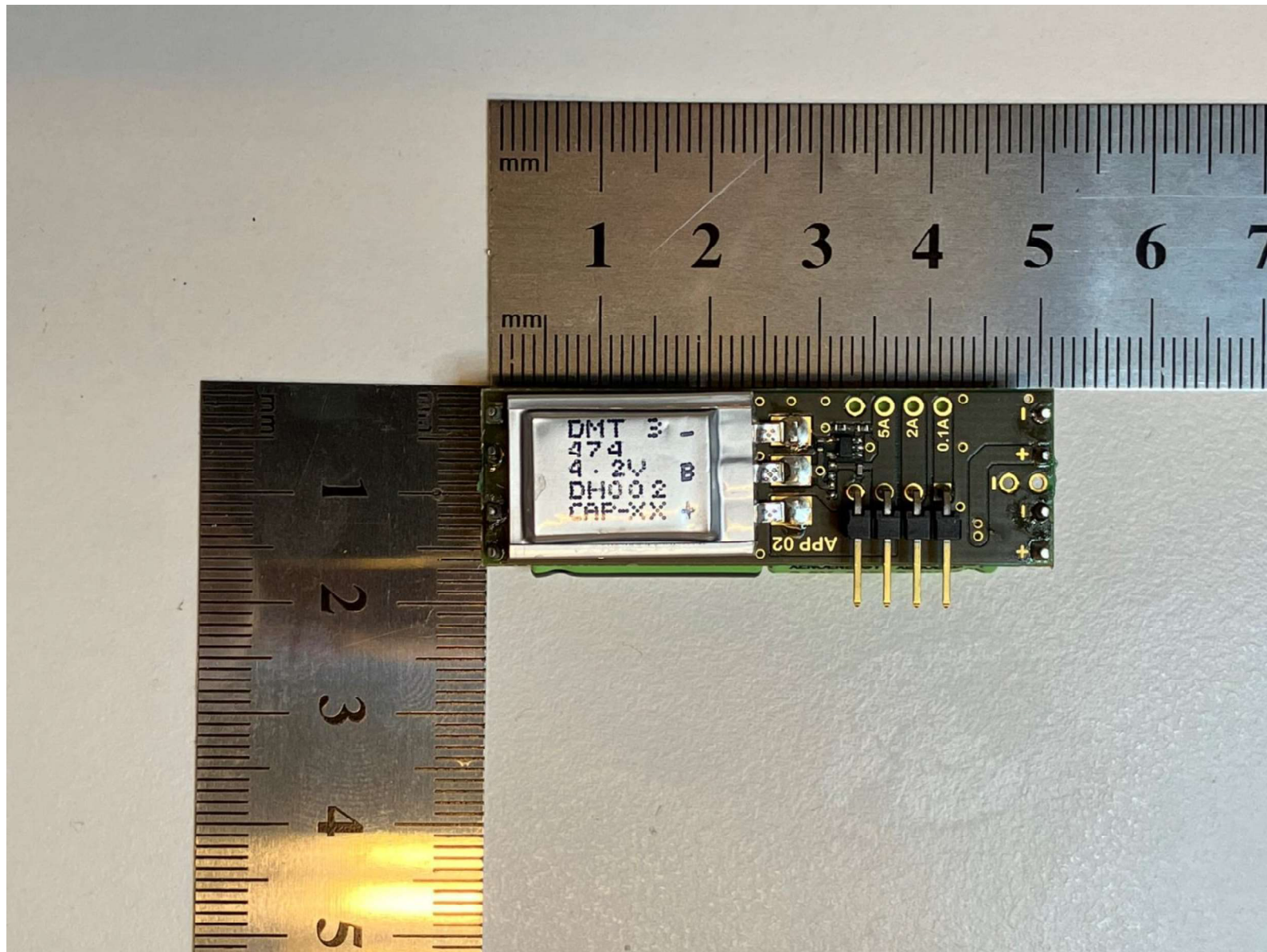
Power pack PCB dimensions
