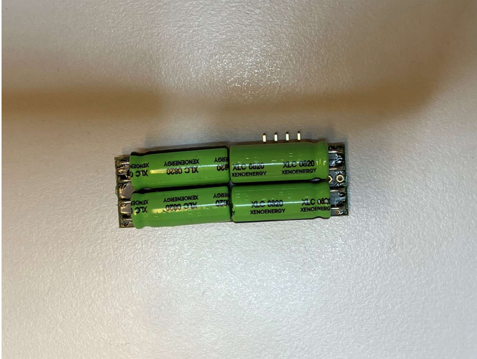
Power pack PCB bottom
