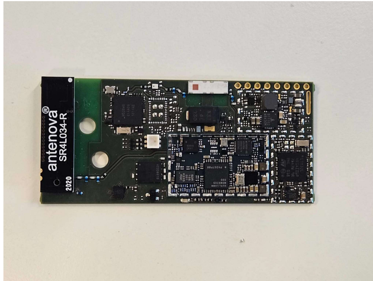
Main PCB top without shields
