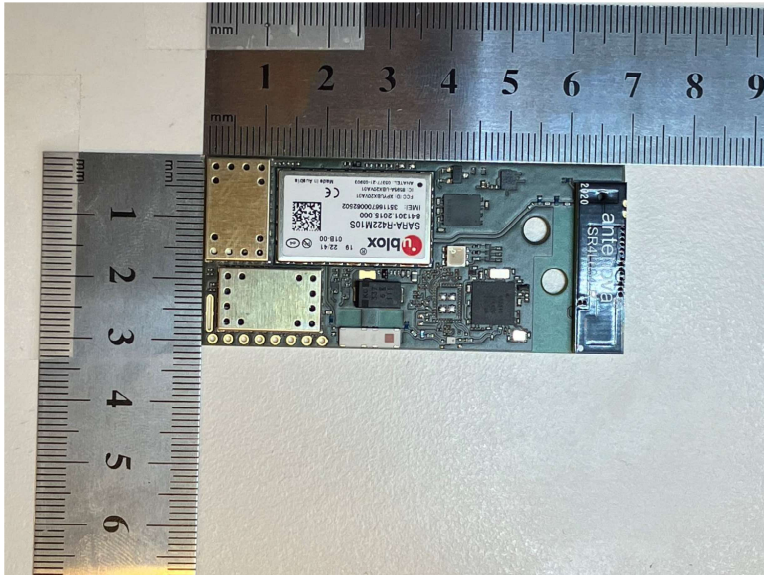
Main PCB dimensions
