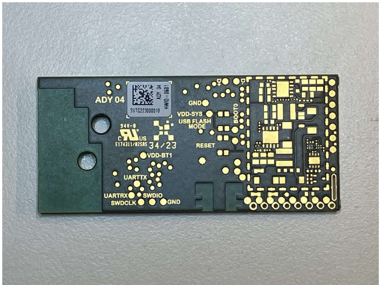
Main PCB bottom
