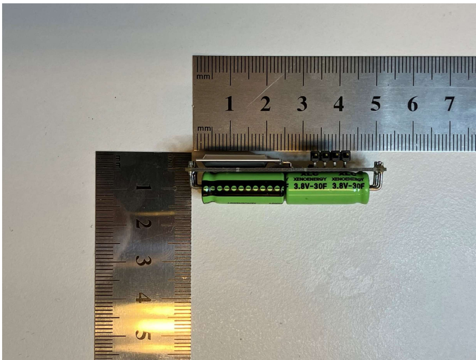
Power pack PCB height
