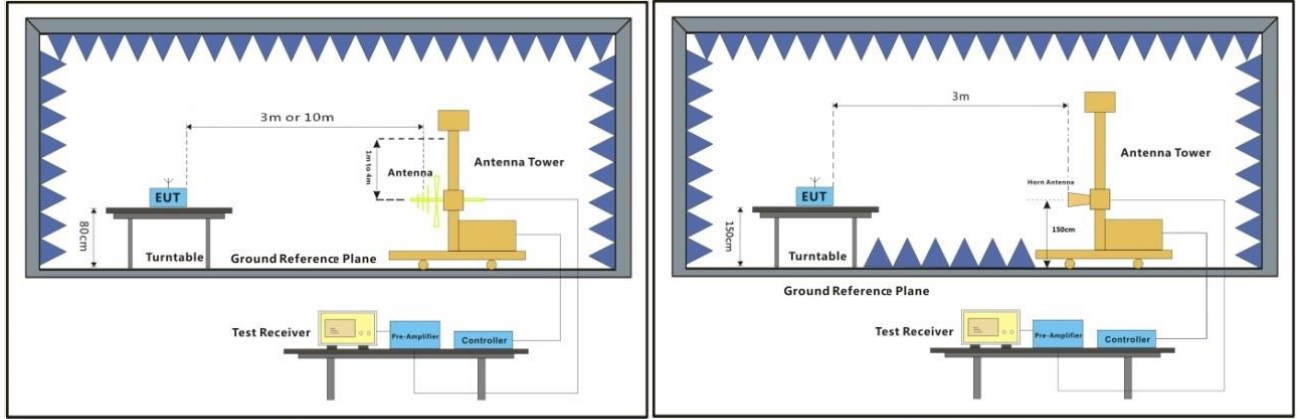
30MHz-1GHz
