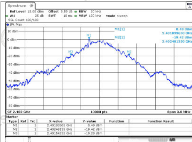
GFSK_DH5_Channel 0
