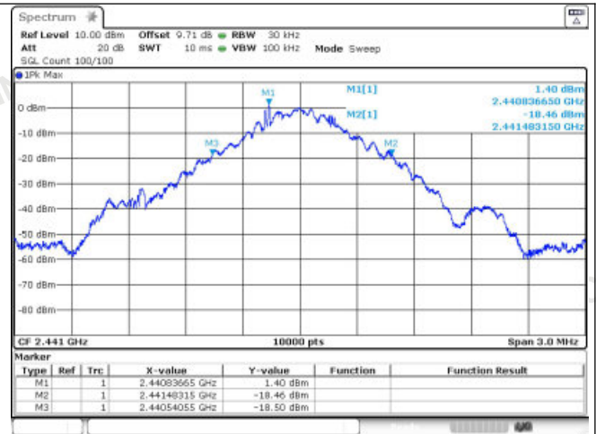
GFSK_DH5_Channel 39
