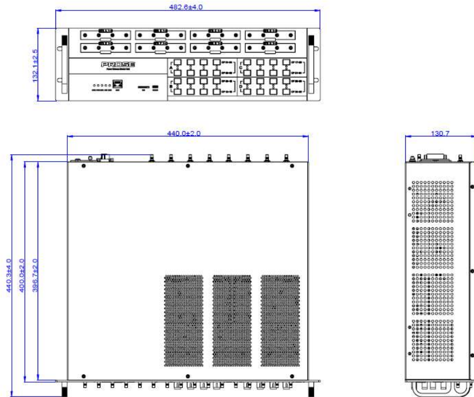
Figure 2-2 PBMU dimensions
