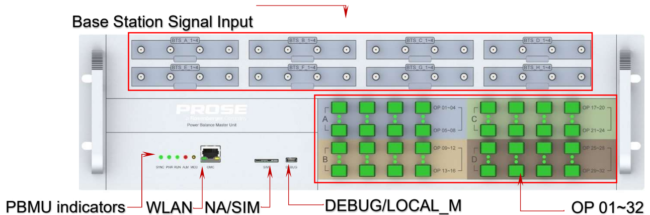
Figure 2-3 (a) Ports in the PBMU front panel
