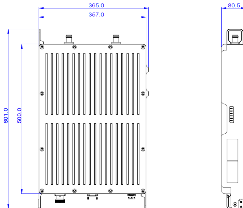
Figure 3-15 LPA dimensions
