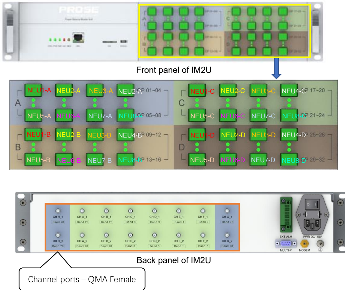
Figure 4-29 IM2U Ports
