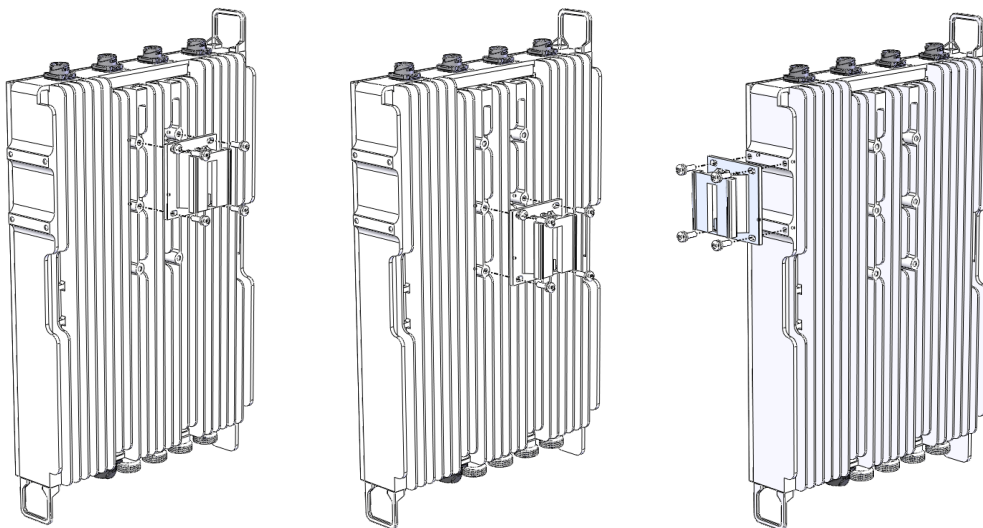
Figure 4-12 Fixed bracket on the equipment
