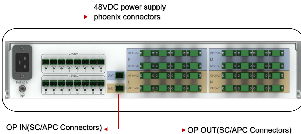
Figure 2-12 Ports in the NEU (NEU-2F32F-XX) rear panel
