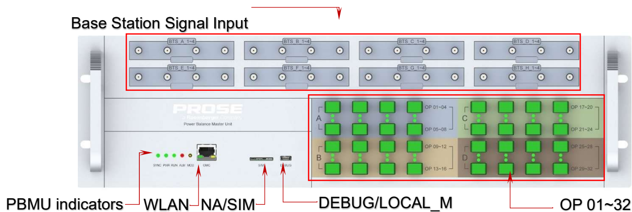
Figure 2-3 (a) Ports in the PBMU front panel
