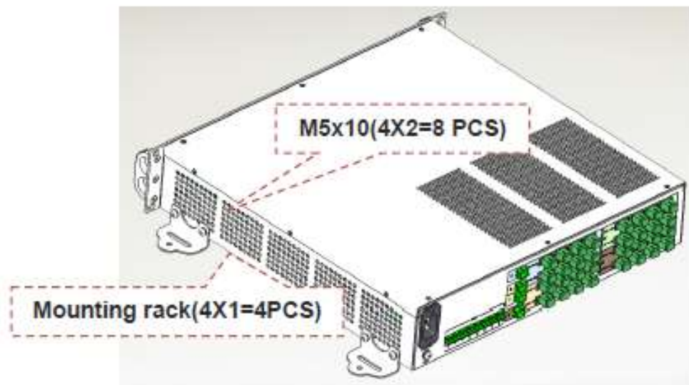
Figure 3-10 Install the mounting support rack
