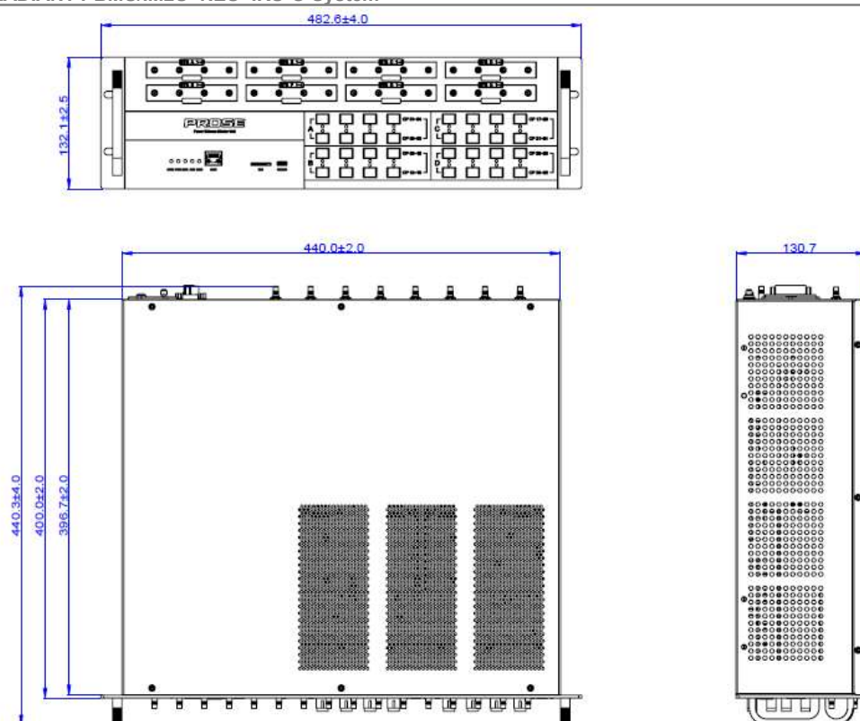
Figure 2-2 PBMU dimensions
