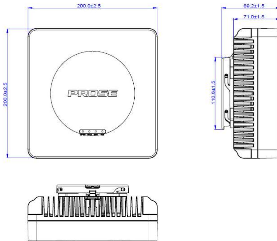
Figure 2-14 IRU-O dimensions
