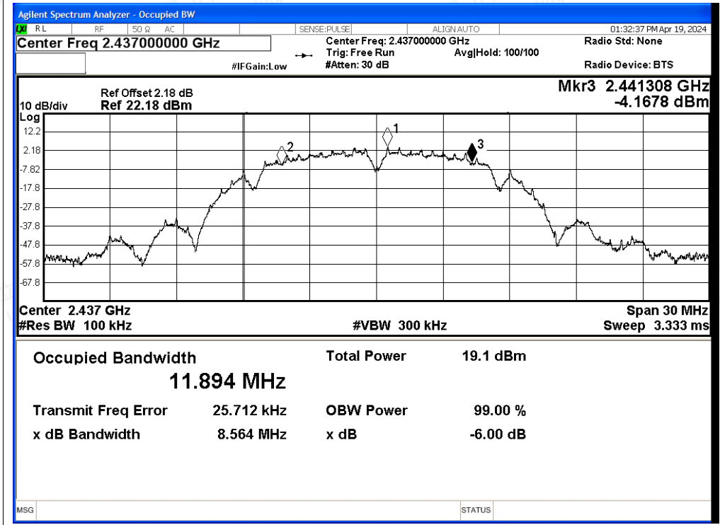
-6dB Bandwidth NVNT b 2437MHz Ant2
