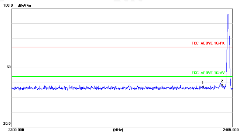
2402MHz Horizontal
