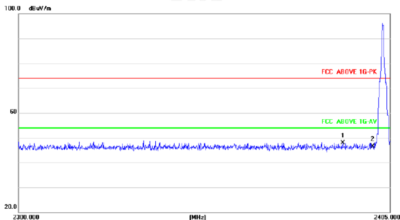
2402MHz Vertical
