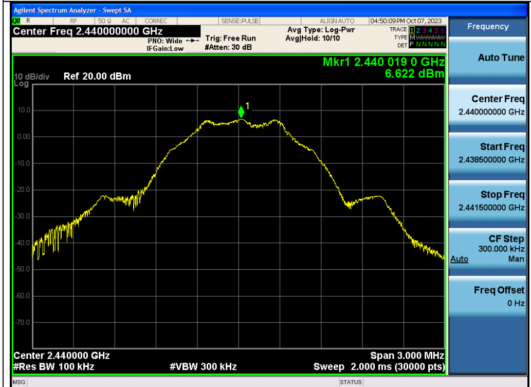
Test_Graph_LE1M_ANT1_2440_1Mbps_Reference Level
