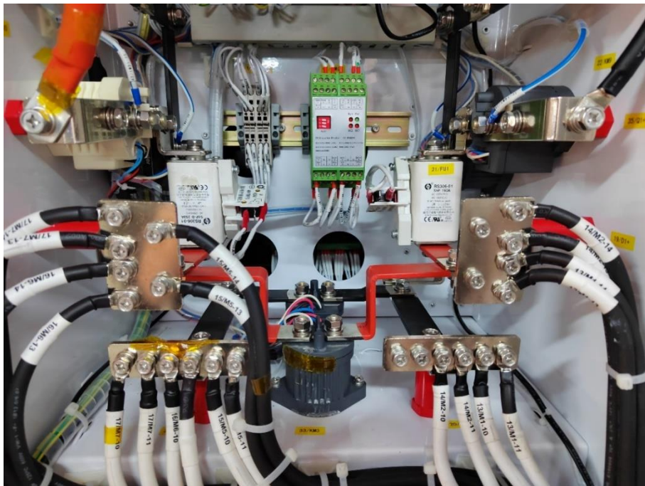
DC output view
