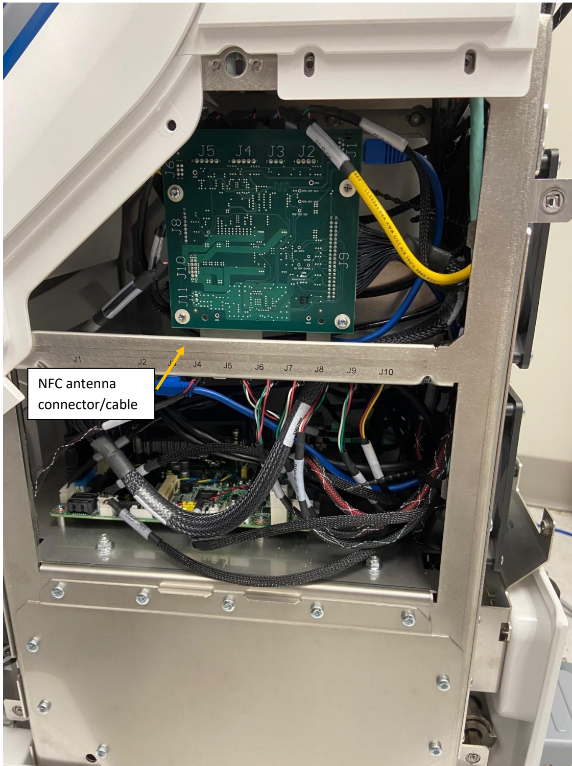
Figure 4: Location of Roller Pump PCA and antenna cable connector in console.
