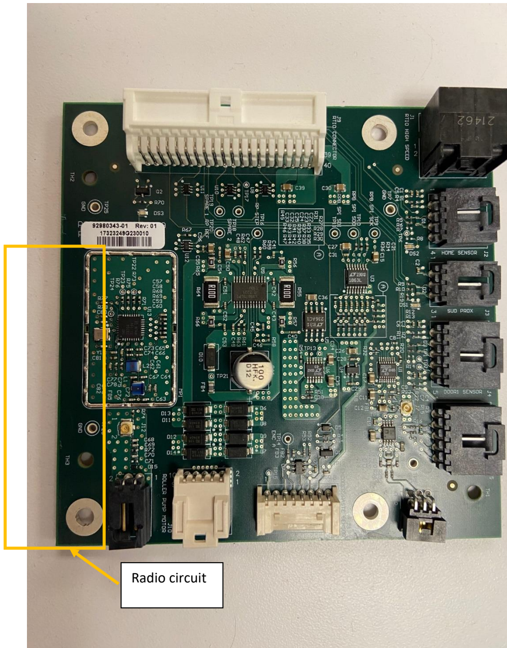
Figure 1: Roller Pump PCA – RFID/NFC Circuits and antenna harness connector J11 location shown in orange box.
