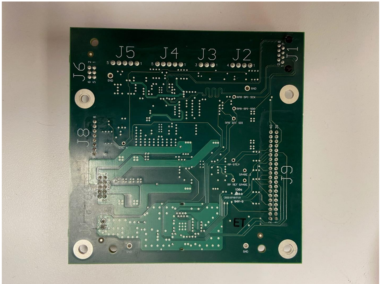
Figure 3: Roller Pump PCA – back side.
