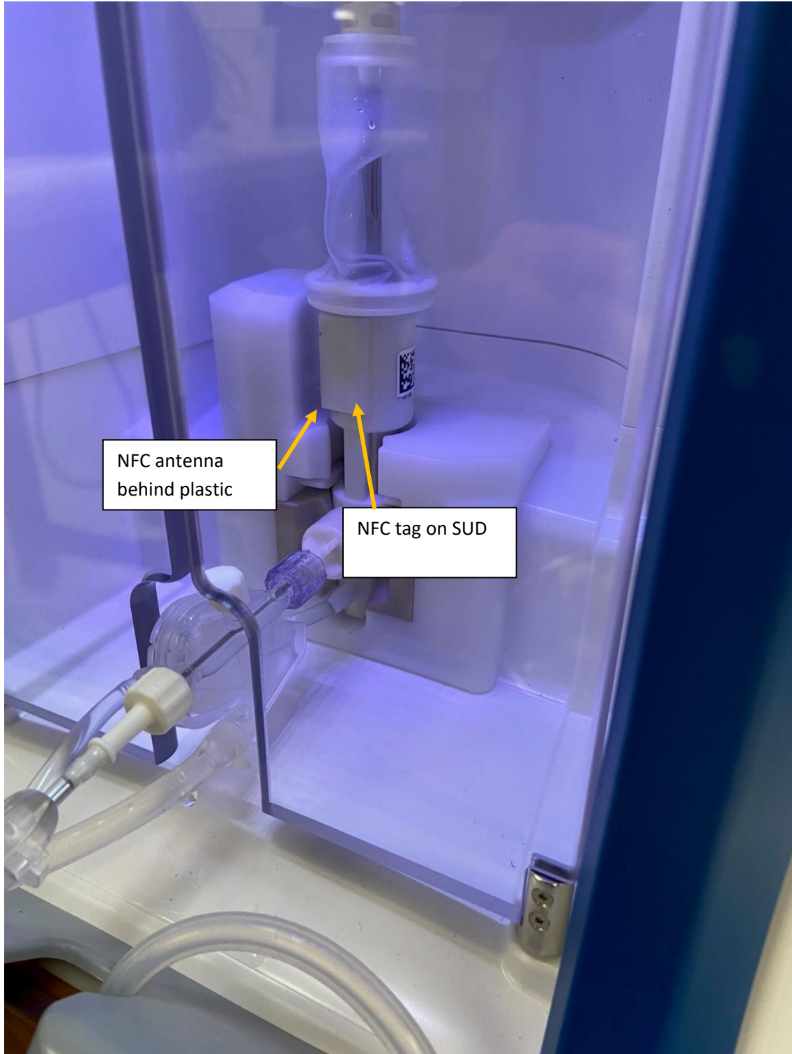
Figure 5: Locations of NFC console antenna and SUD tag in capture bay of console.
