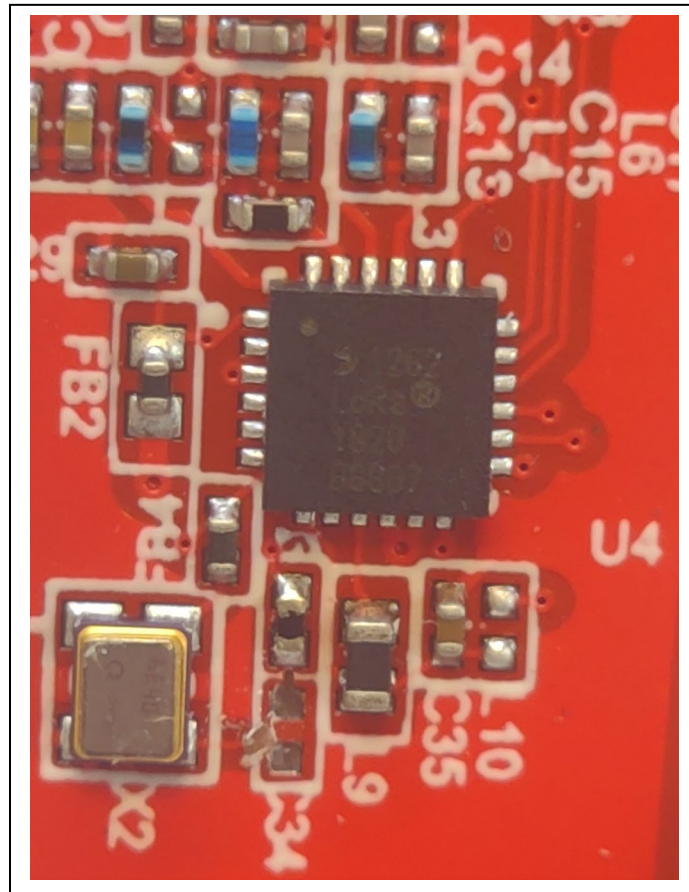
LoRa Chip
