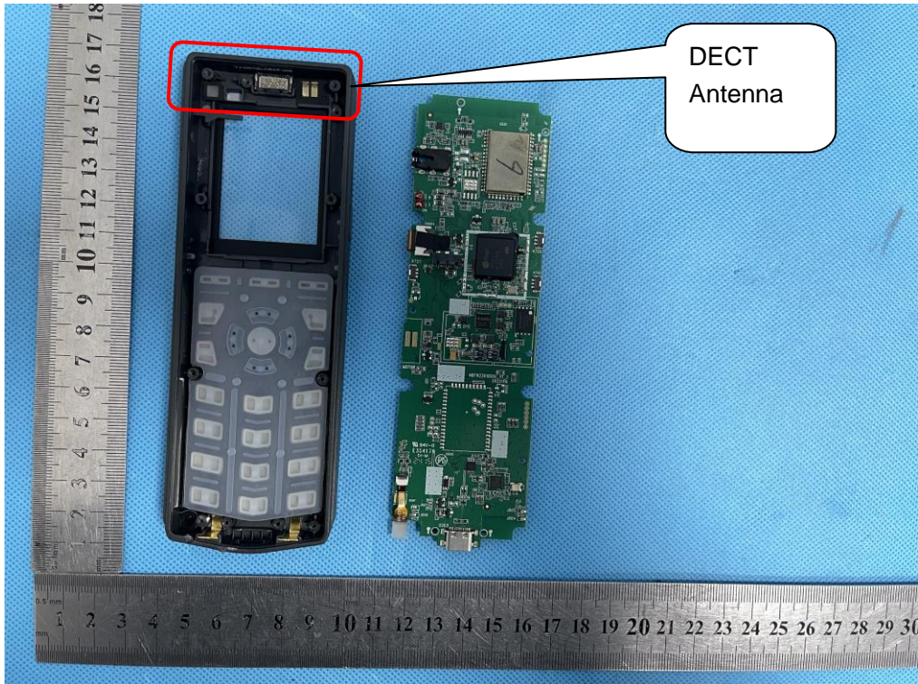
DECT ANTENNA
