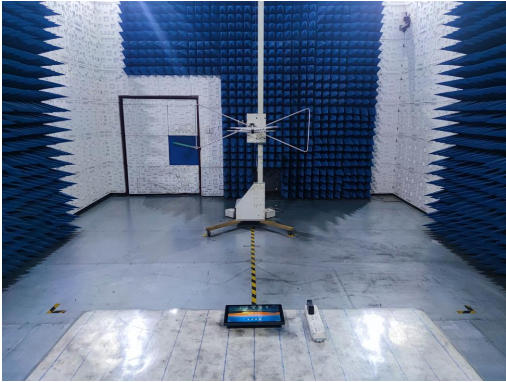
RADIATED EMISSION TEST SETUP BELOW 1GHz-Charging from POE
