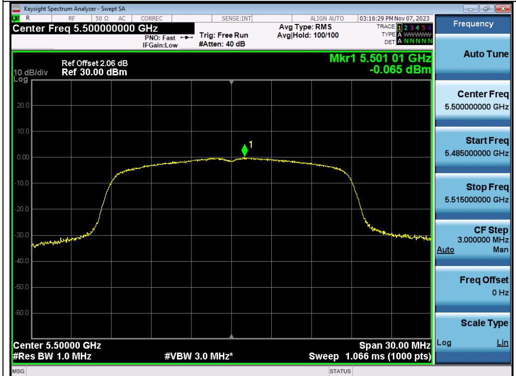
Test_Graph_802.11n20_ANT1_5500_MCS0_PSD
