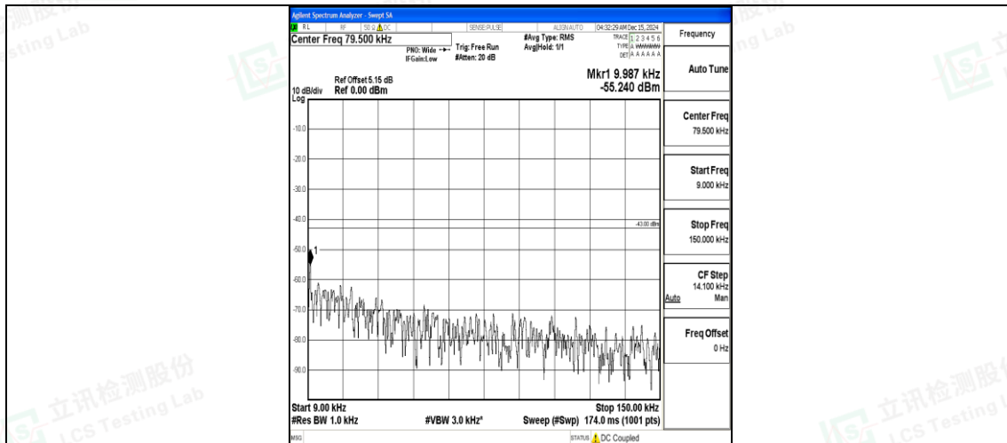
Band66_15MHz_QPSK_132047_1RB#0_0.009~0.15_0.009~0.15
