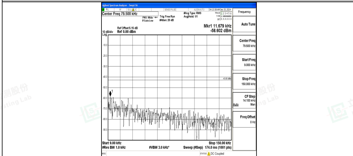
Band66_10MHz_16QAM_132622_1RB#0_0.009~0.15_0.009~0.15
