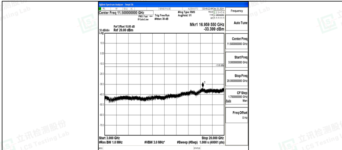
Band66_5MHz_16QAM_131997_1RB#0_3000~20000_3000~20000
