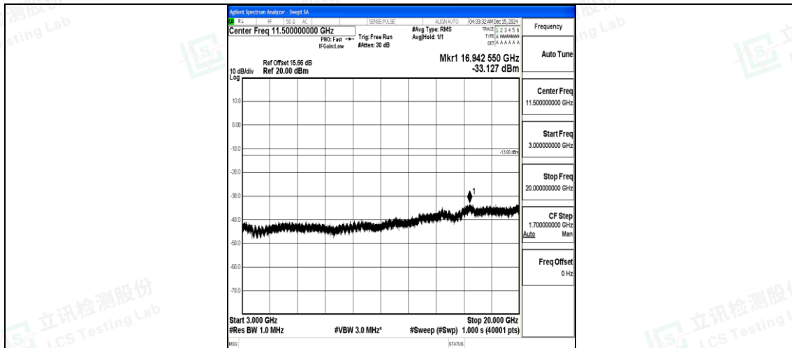
Band66_15MHz_16QAM_132047_1RB#0_3000~20000_3000~20000
