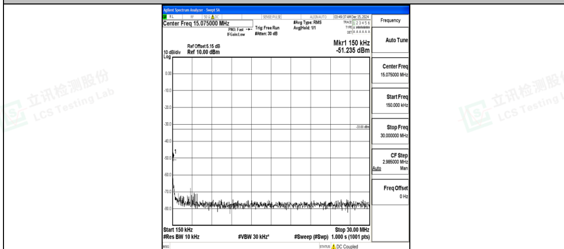
Band66_5MHz_QPSK_132322_1RB#0_0.15~30_0.15~30
