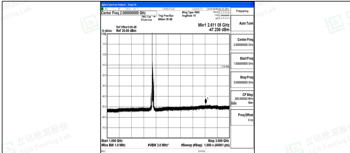
Band66_15MHz_16QAM_132322_1RB#0_1000~3000_1000~3000
