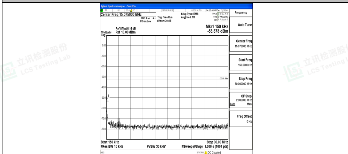
Band66_10MHz_16QAM_132622_1RB#0_0.15~30_0.15~30
