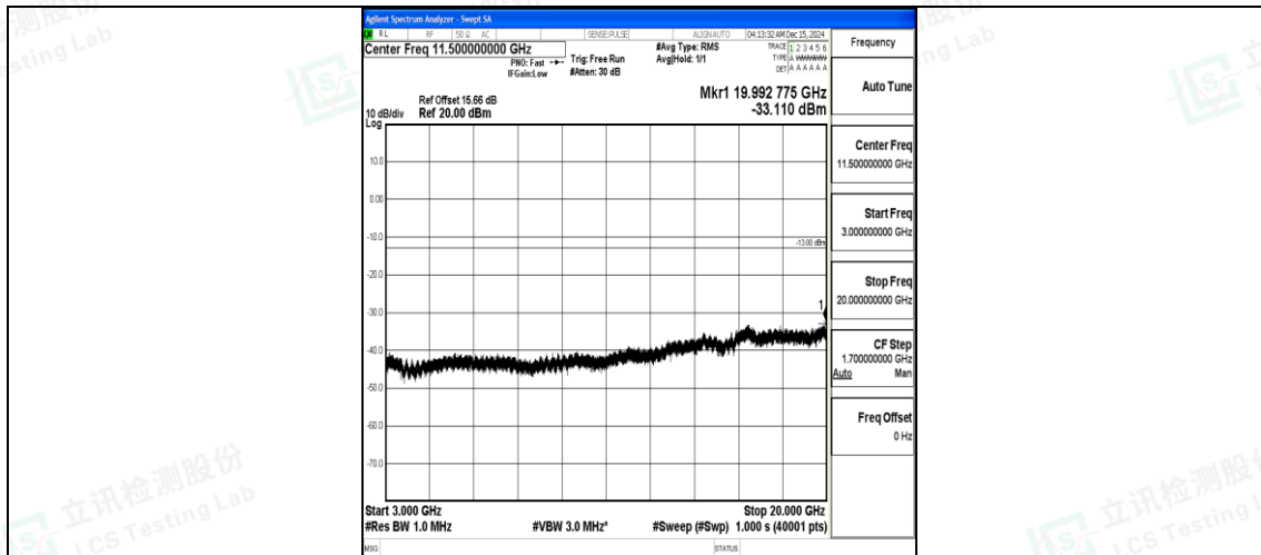
Band66_10MHz_QPSK_132622_1RB#0_3000~20000_3000~20000
