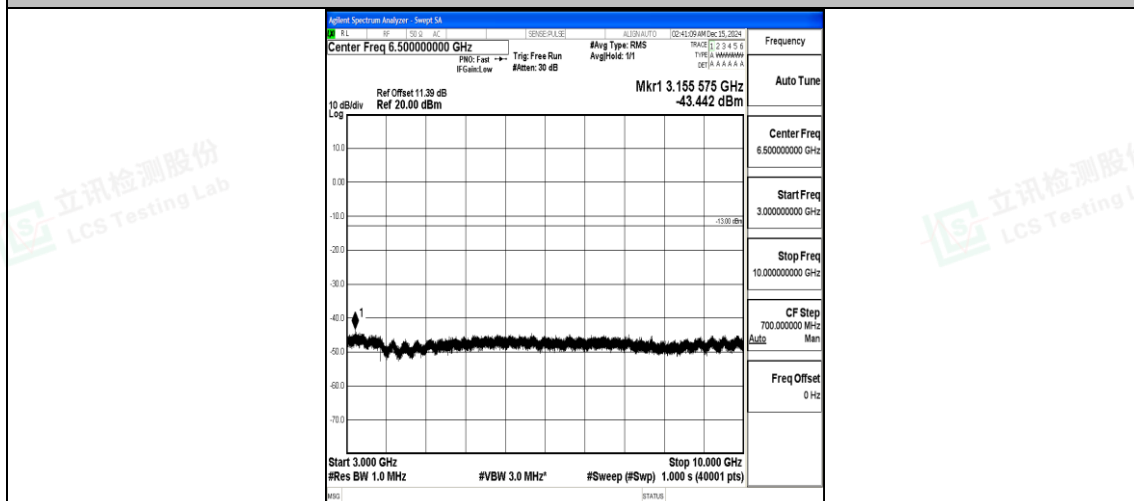
Band26_15MHz_16QAM_26965_1RB#0_3000~10000_3000~10000
