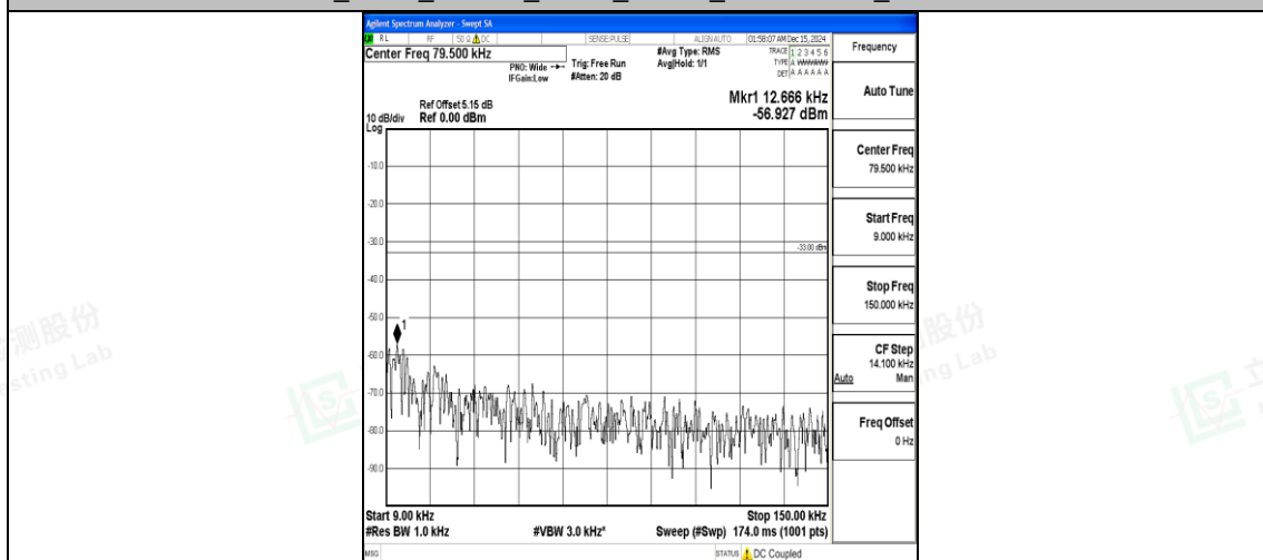
Band26_5MHz_QPSK_26915_1RB#0_0.009~0.15_0.009~0.15
