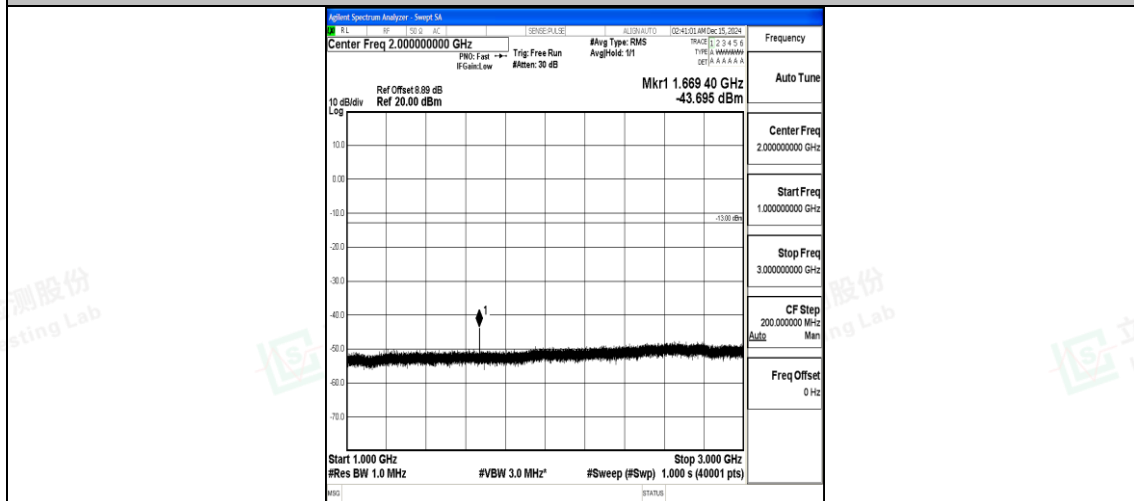
Band26_15MHz_16QAM_26965_1RB#0_1000~3000_1000~3000
