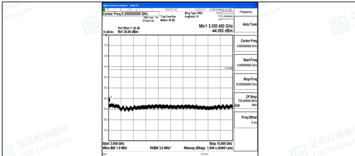
Band26_5MHz_QPSK_27015_1RB#0_3000~10000_3000~10000
