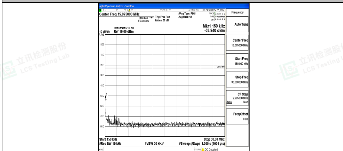
Band26_5MHz_16QAM_27015_1RB#0_0.15~30_0.15~30
