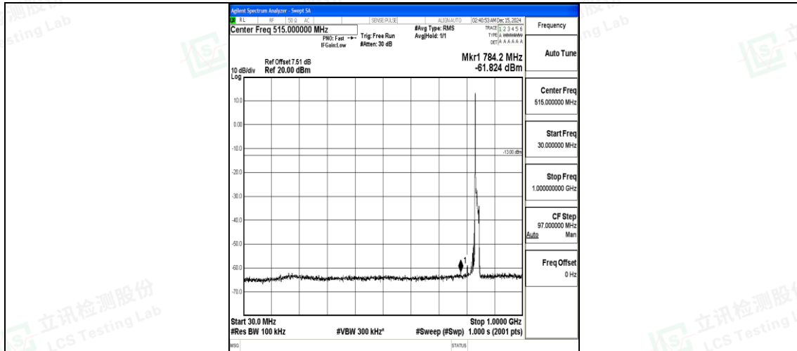
Band26_15MHz_16QAM_26965_1RB#0_30~1000_30~1000
