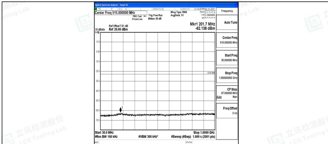
Band25_15MHz_16QAM_26615_1RB#0_30~1000_30~1000
