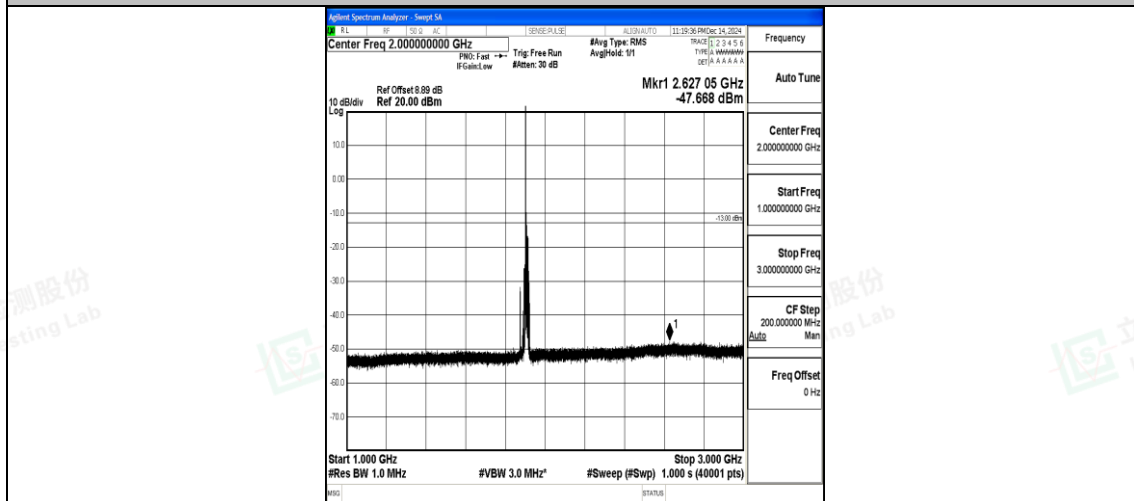
Band25_15MHz_16QAM_26615_1RB#0_1000~3000_1000~3000
