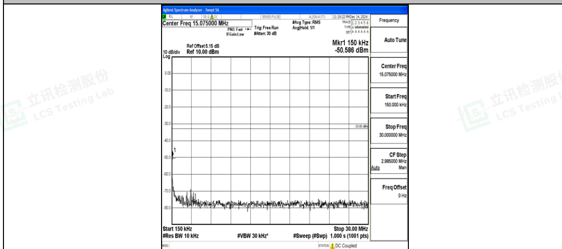
Band25_15MHz_16QAM_26615_1RB#0_0.15~30_0.15~30
