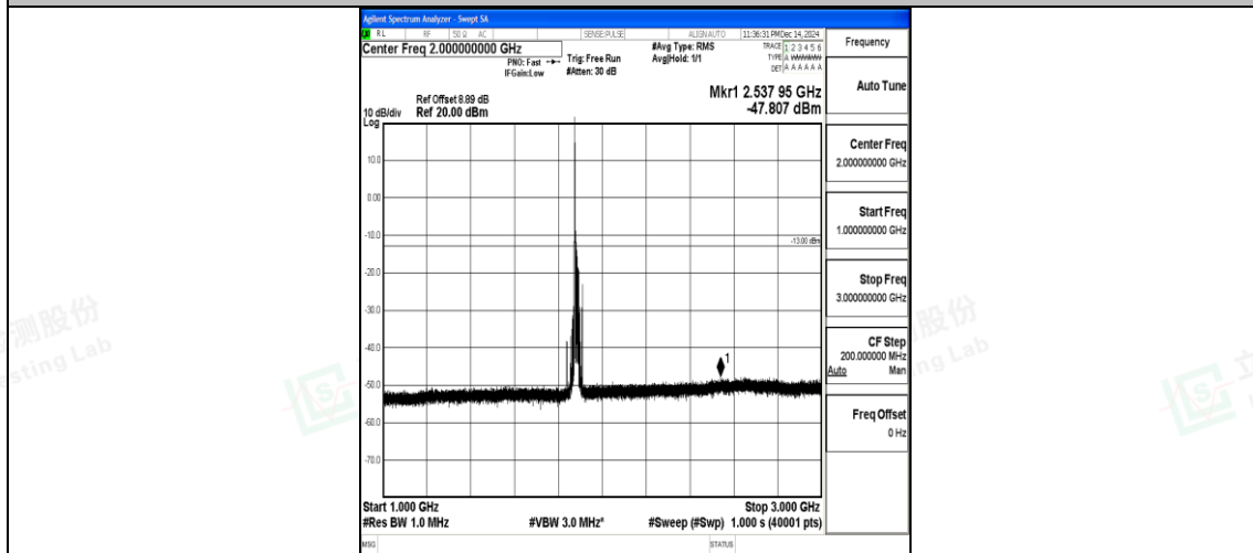
Band25_20MHz_QPSK_26365_1RB#0_1000~3000_1000~3000
