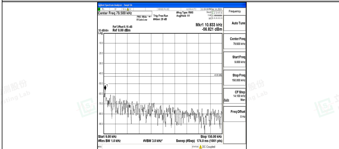
Band25_15MHz_16QAM_26615_1RB#0_0.009~0.15_0.009~0.15
