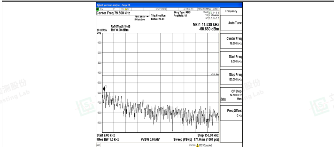
Band25_1.4MHz_QPSK_26365_1RB#0_0.009~0.15_0.009~0.15
