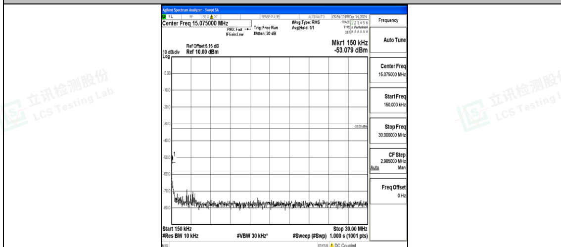
Band25_1.4MHz_QPSK_26365_1RB#0_0.15~30_0.15~30
