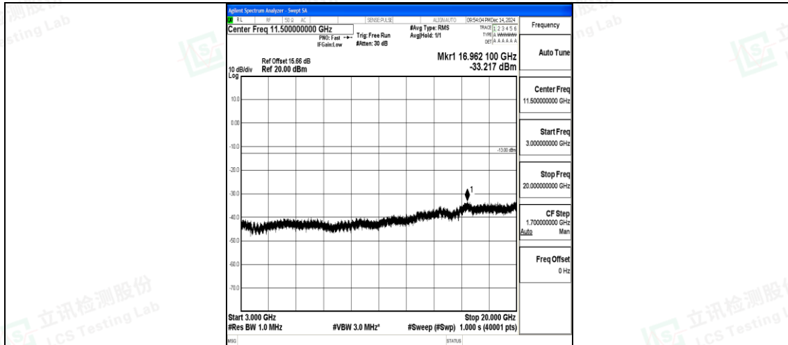
Band25_1.4MHz_16QAM_26047_1RB#0_3000~20000_3000~20000
