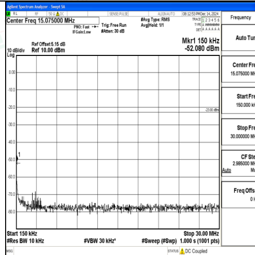
Band12_5MHz_QPSK_23095_1RB#0_0.15~30_0.15~30
