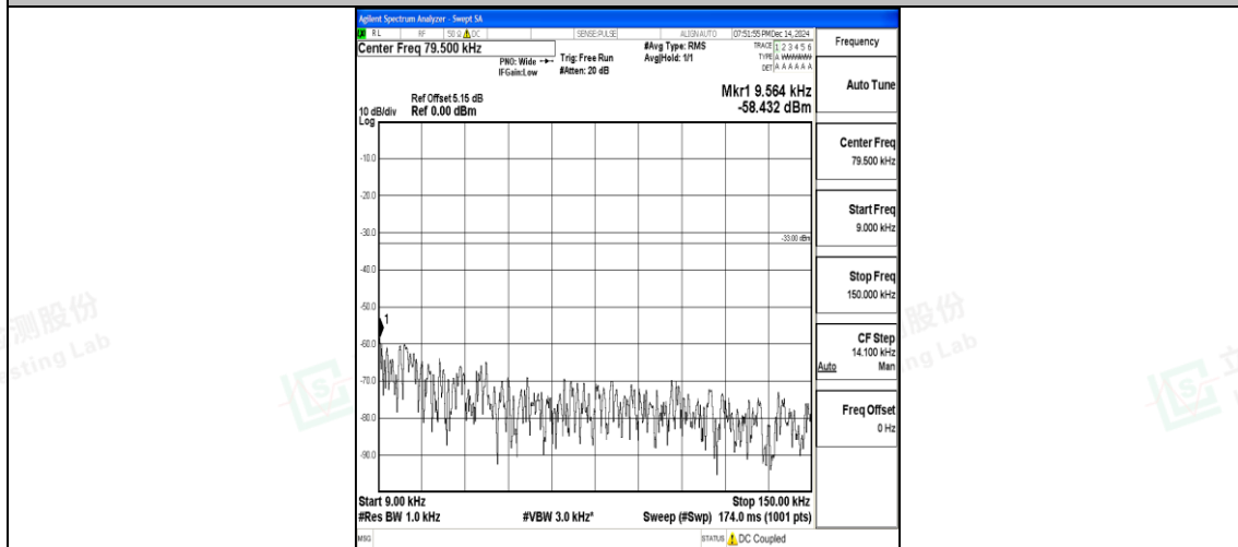
Band12_3MHz_QPSK_23025_1RB#0_0.009~0.15_0.009~0.15
