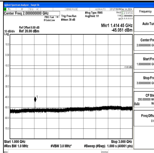
Band12_1.4MHz_QPSK_23095_1RB#0_1000~3000_1000~3000
