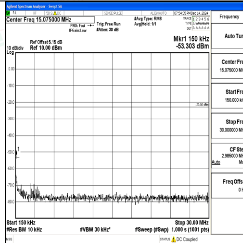
Band12_3MHz_16QAM_23165_1RB#0_0.15~30_0.15~30
