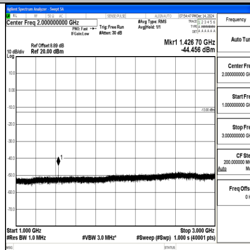
Band12_3MHz_16QAM_23165_1RB#0_1000~3000_1000~3000
