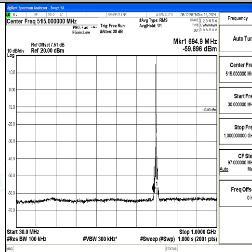
Band12_5MHz_QPSK_23095_1RB#0_30~1000_30~1000
