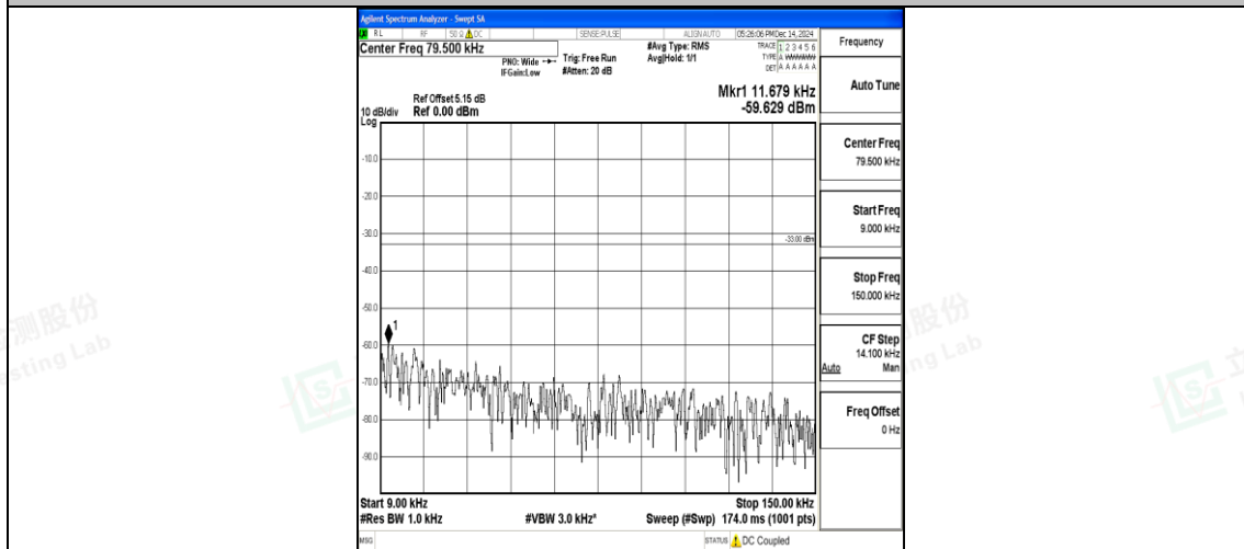
Band5_3MHz_QPSK_20415_1RB#0_0.009~0.15_0.009~0.15
