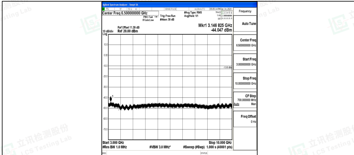
Band5_1.4MHz_16QAM_20643_1RB#0_3000~10000_3000~10000
