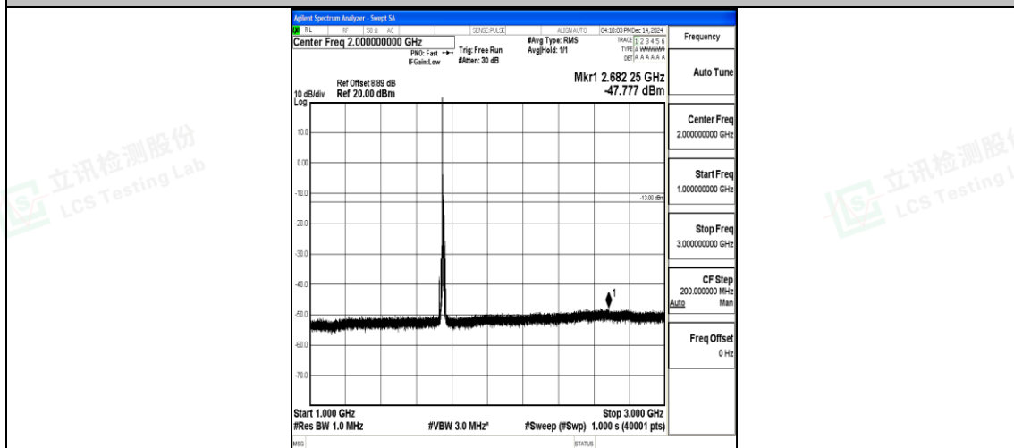
Band4_10MHz_QPSK_20350_1RB#0_1000~3000_1000~3000
