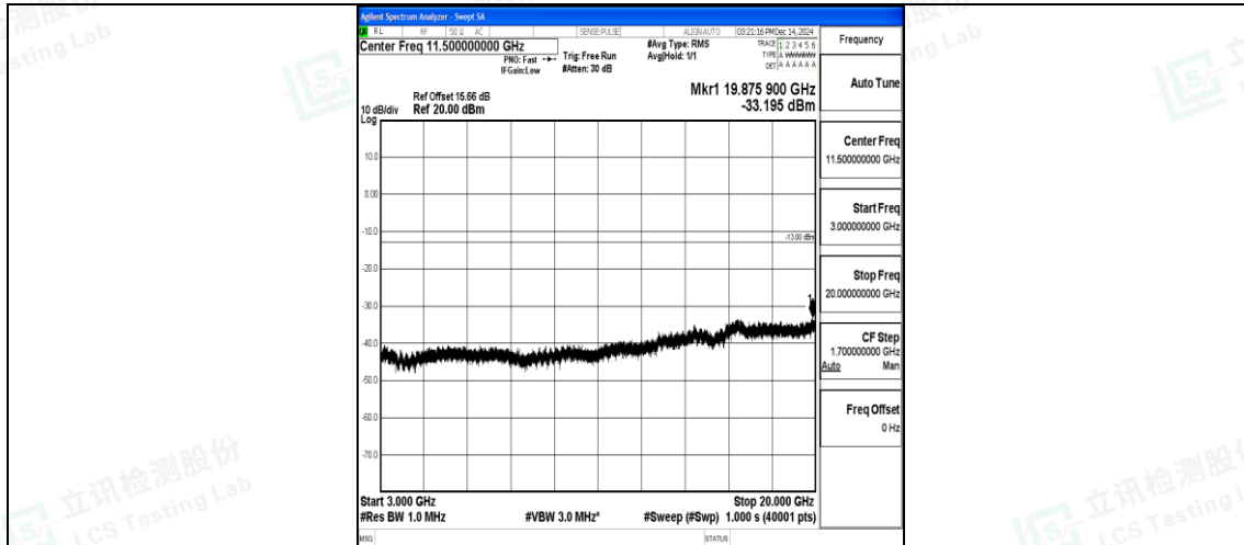
Band4_1.4MHz_QPSK_20393_1RB#0_3000~20000_3000~20000
