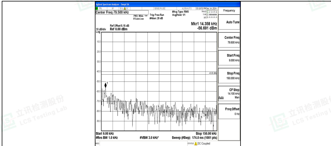
Band4_1.4MHz_QPSK_19957_1RB#0_0.009~0.15_0.009~0.15
