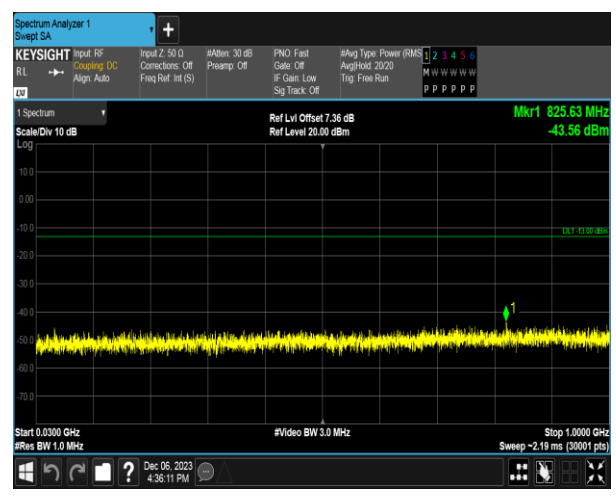
WCDMA 1900_HSDPA_HCH
