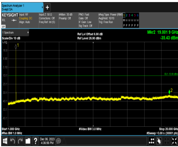
WCDMA 1900_HSDPA_HCH
