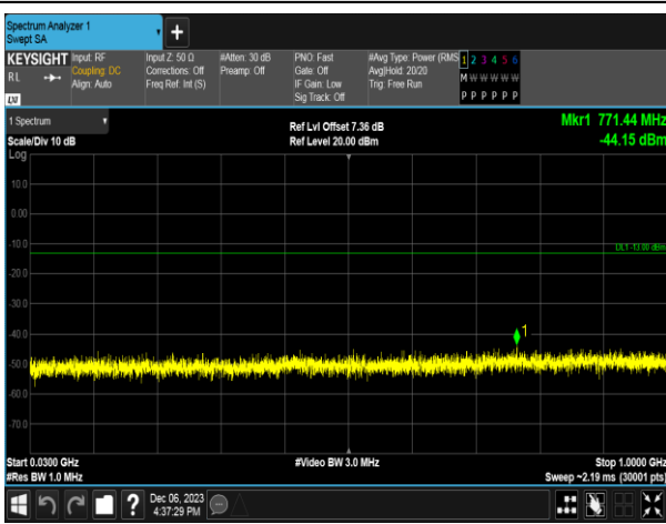
WCDMA 1900_HSDPA_HCH
