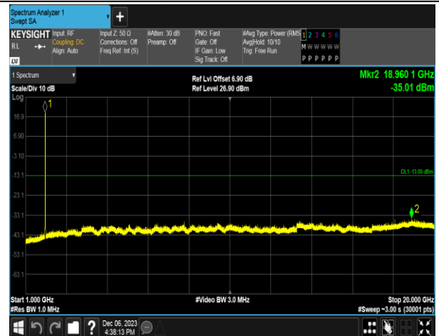
WCDMA 1900_HSDPA_HCH
