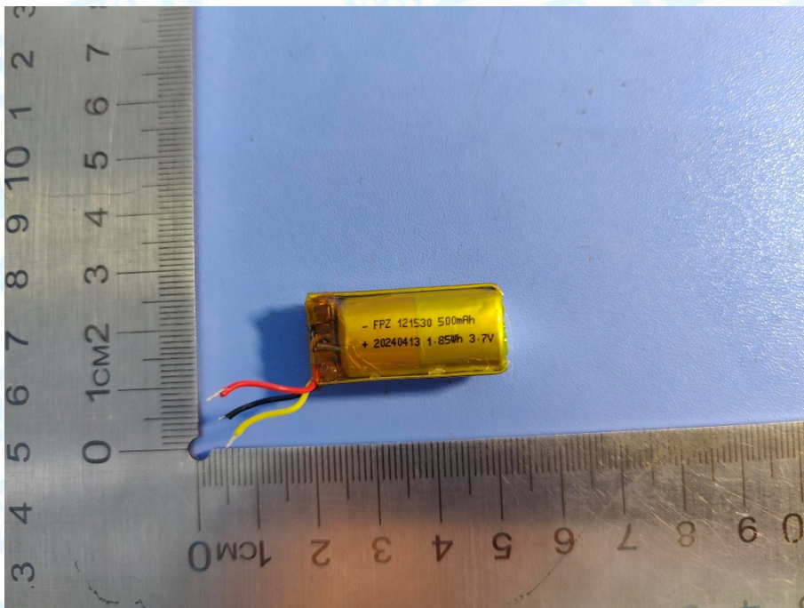
Photo 15 Battery Appearance
