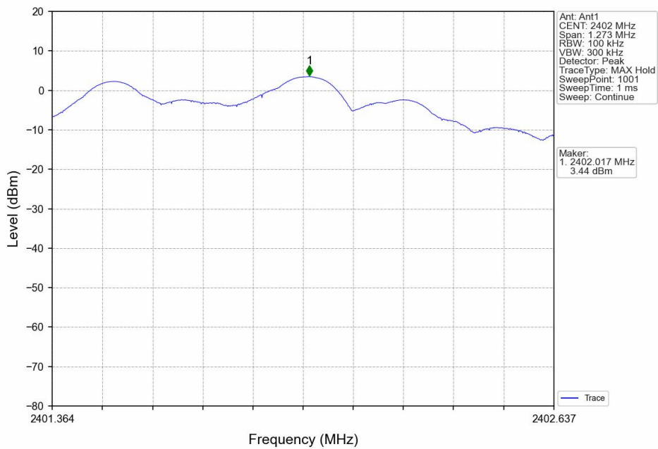
2M_LCH_2402MHz
