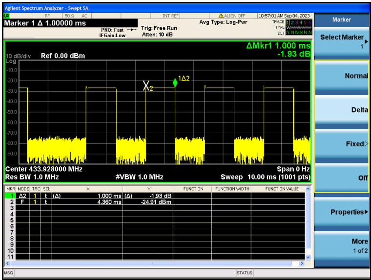
(Time per burst: 1.000ms*9pcs)
