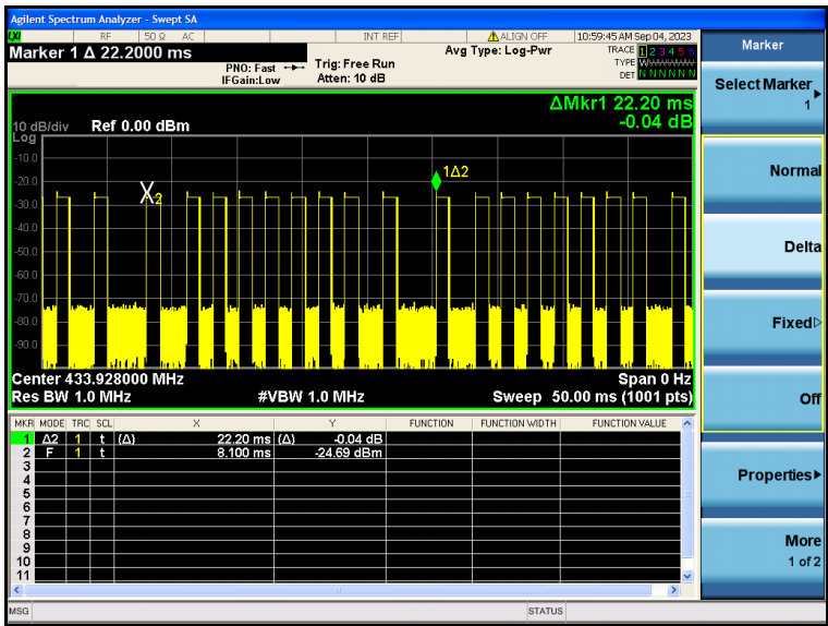
(Transmit cycle 22.20ms)
