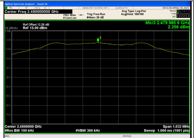
In-Band Reference Level LE Channel 39
