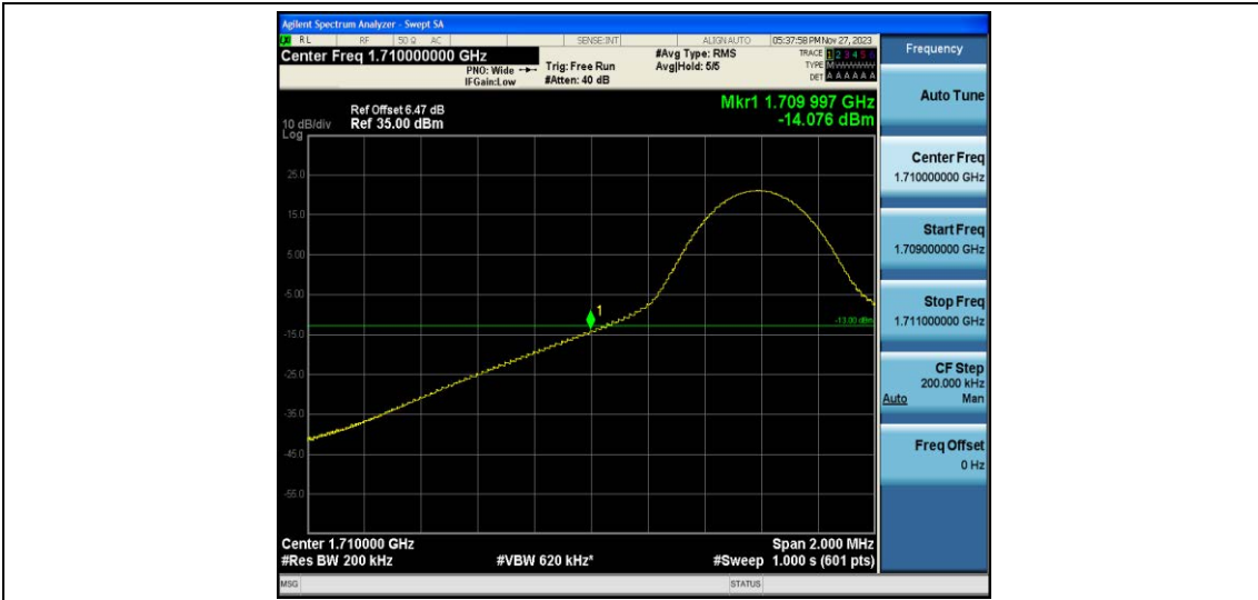
Band66-10MHz-QPSK-132022-1RB#49
