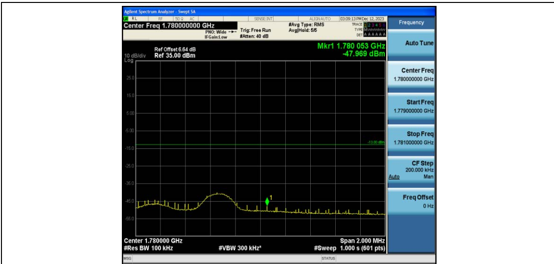
Band66-5MHz-QPSK-132647-1RB#24
