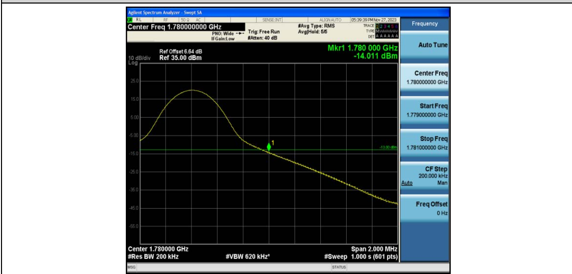
Band66-10MHz-QPSK-132622-50RB#0
