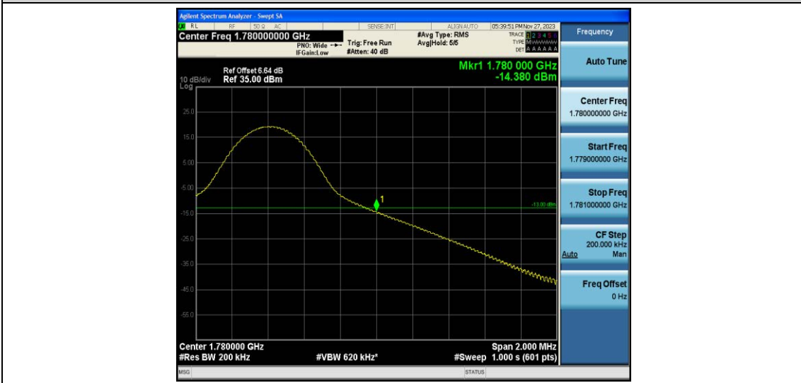
Band66-10MHz-16QAM-132622-50RB#0
