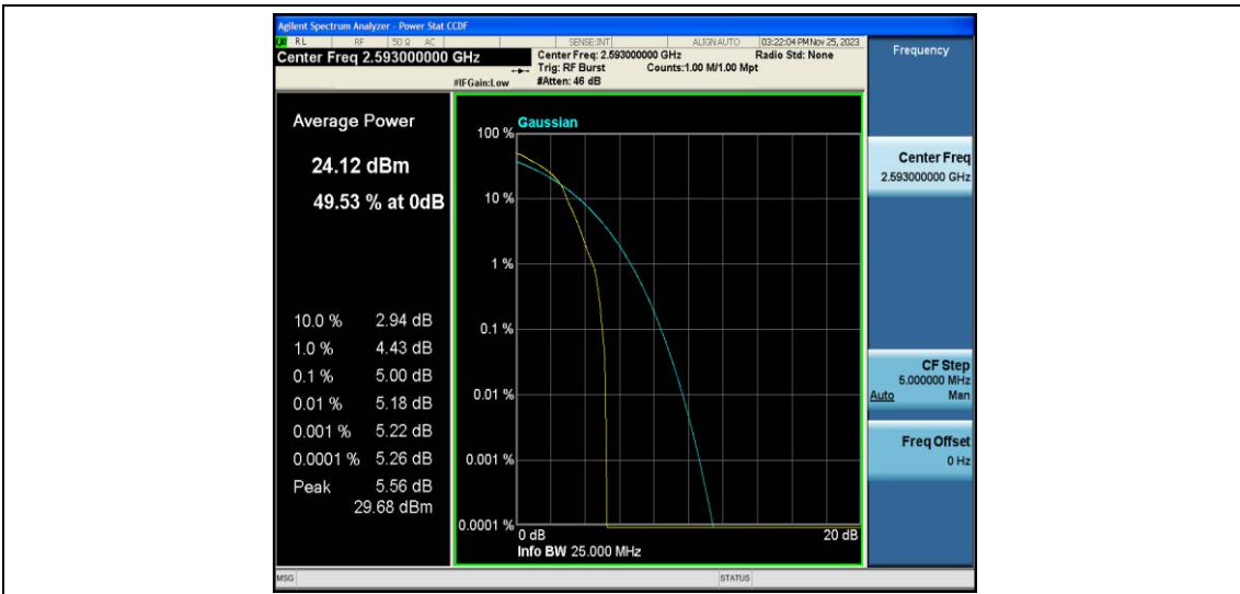
Band41-5MHz-16QAM-40620-25RB#0
