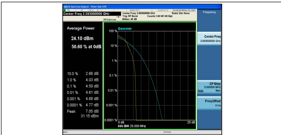
Band41-20MHz-16QAM-40620-100RB#0
