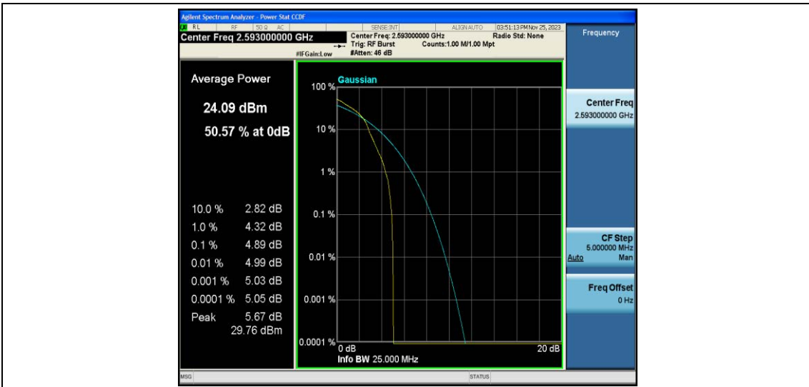
Band41-15MHz-16QAM-40620-75RB#0
