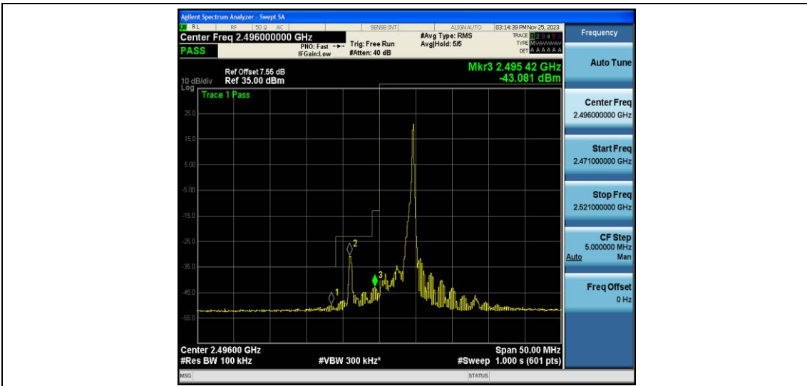
Band41-5MHz-QPSK-39675-25RB#0
