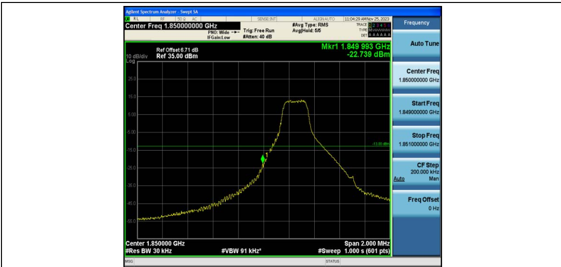
Band25-1.4MHz-16QAM-26047-1RB#5
