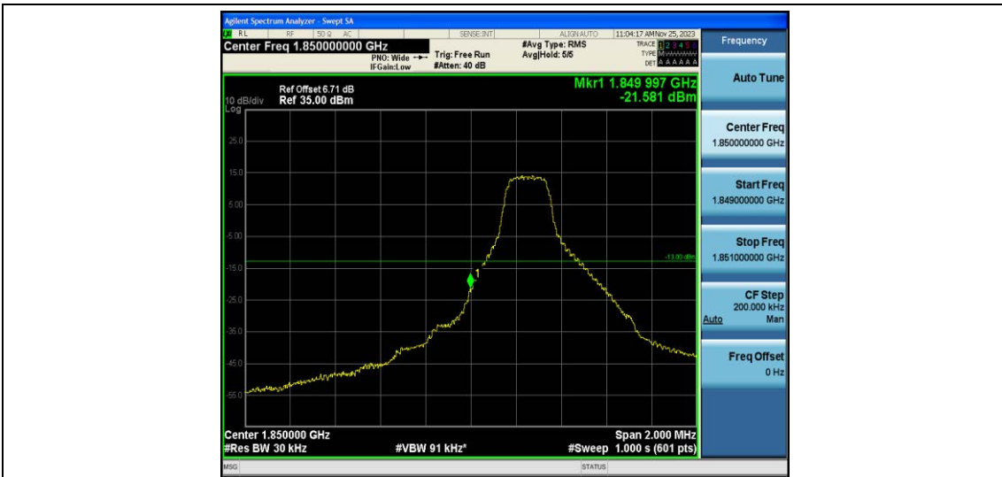
Band25-1.4MHz-QPSK-26047-1RB#5
