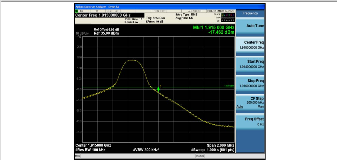
Band25-5MHz-QPSK-26665-25RB#0
