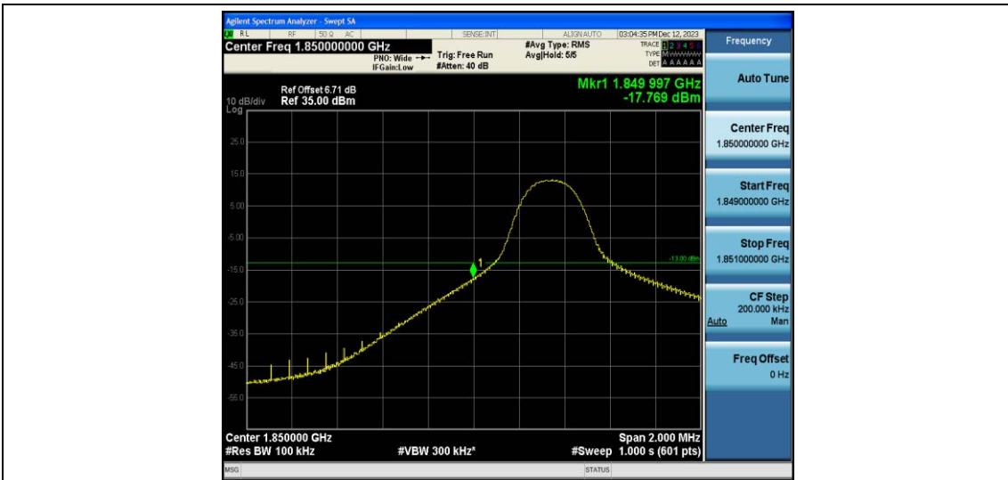
Band25-5MHz-QPSK-26065-1RB#24
