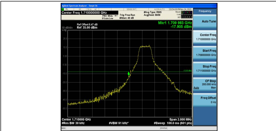
Band4-1.4MHz-16QAM-19957-1RB#5
