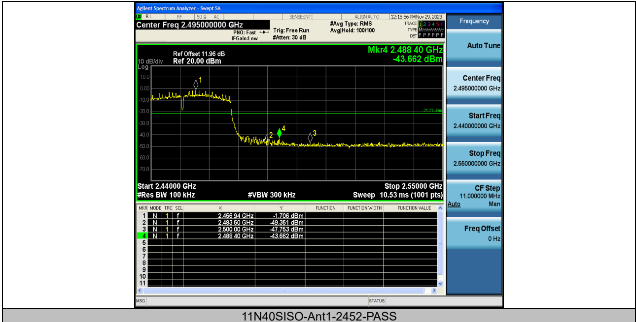
11N40SISO-Ant1-2452-PASS
