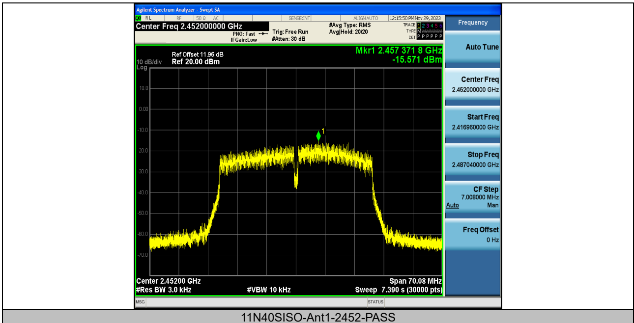
11N40SISO-Ant1-2452-PASS
