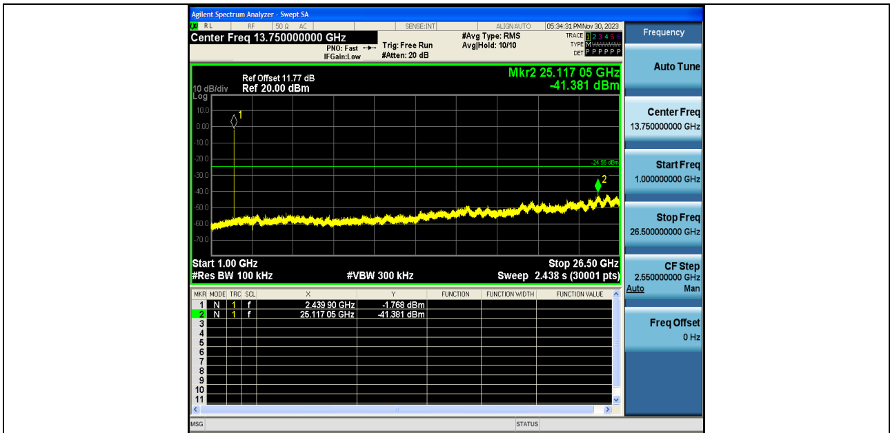
BLE_2M-Ant1-2440-1000~26500-PASS
