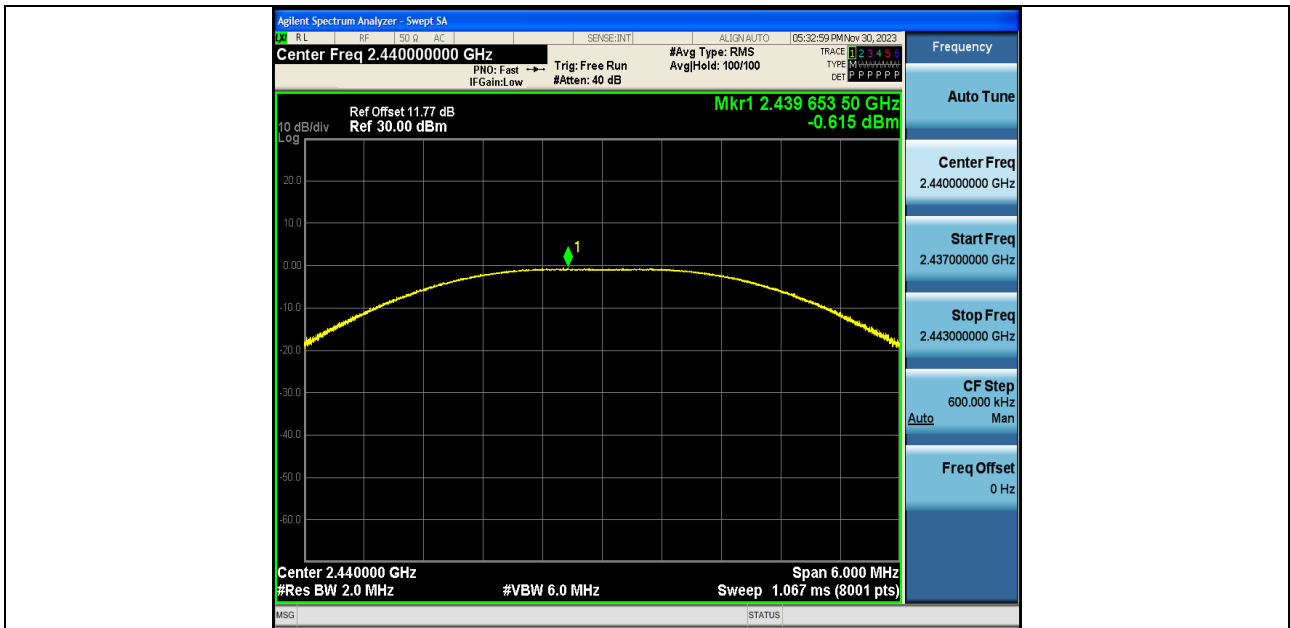
BLE_2M-Ant1-2440-PASS
