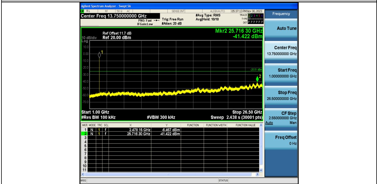
BLE_2M-Ant1-2478-1000~26500-PASS
