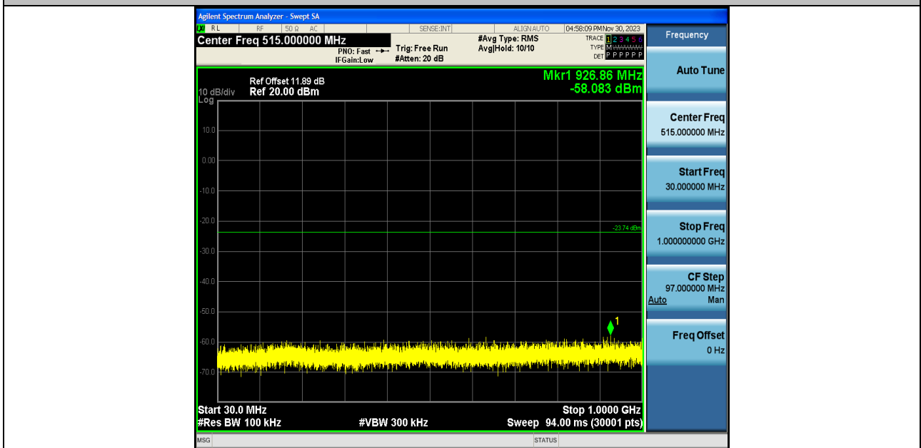
BLE_1M-Ant1-2402-30~1000-PASS
