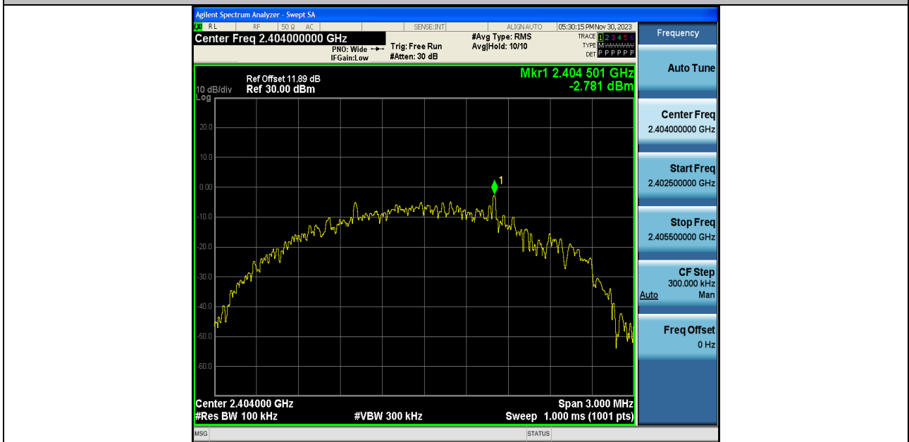
BLE_2M-Ant1-2404-0~Reference-PASS
