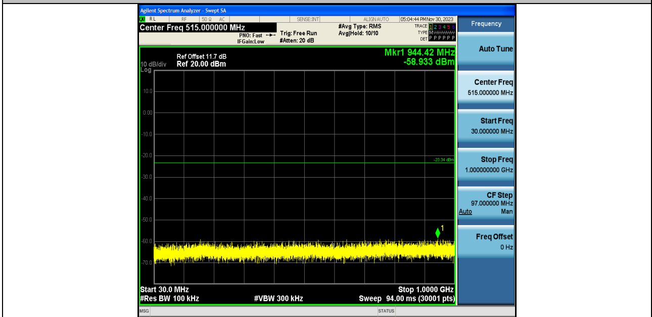
BLE_1M-Ant1-2480-30~1000-PASS
