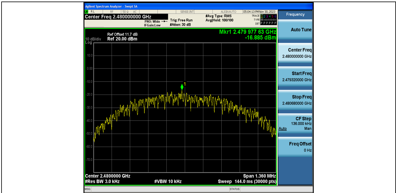
BLE_1M-Ant1-2480-PASS
