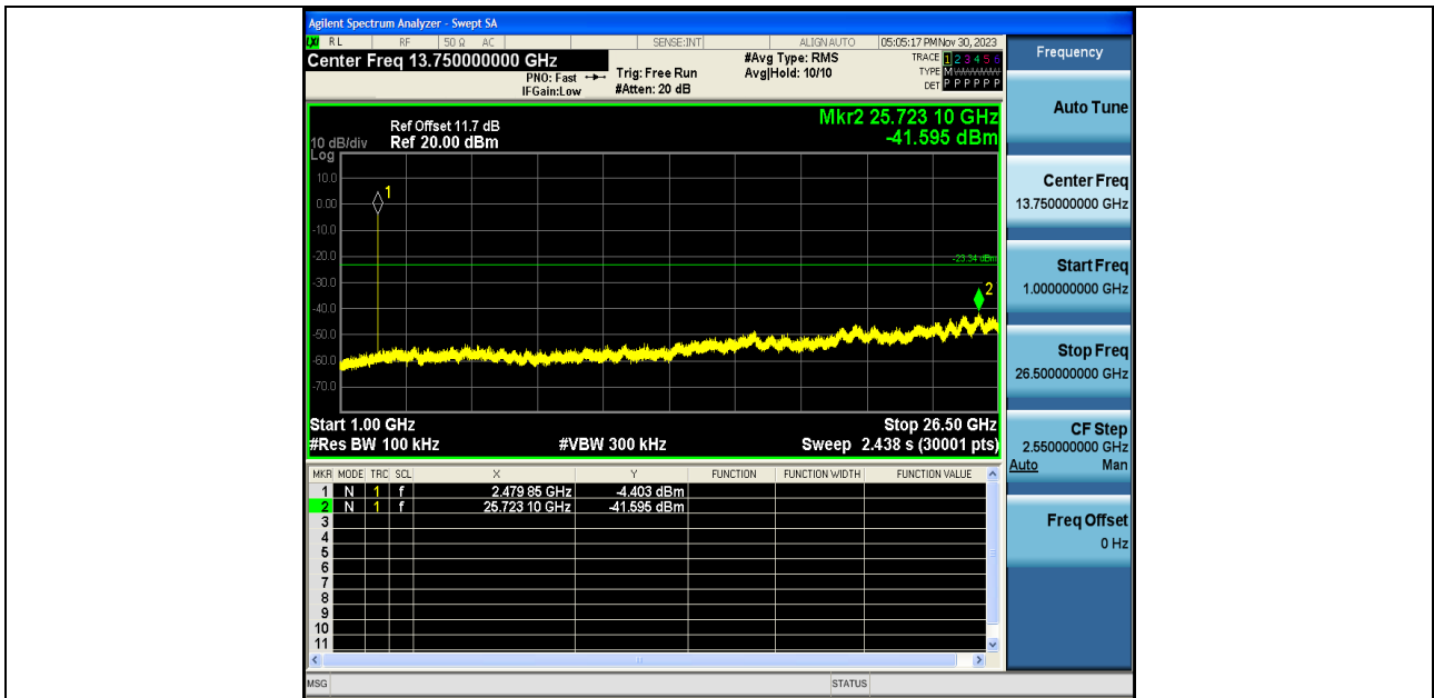
BLE_1M-Ant1-2480-1000~26500-PASS
