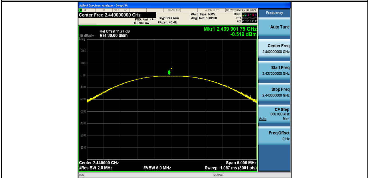
BLE_1M-Ant1-2440-PASS
