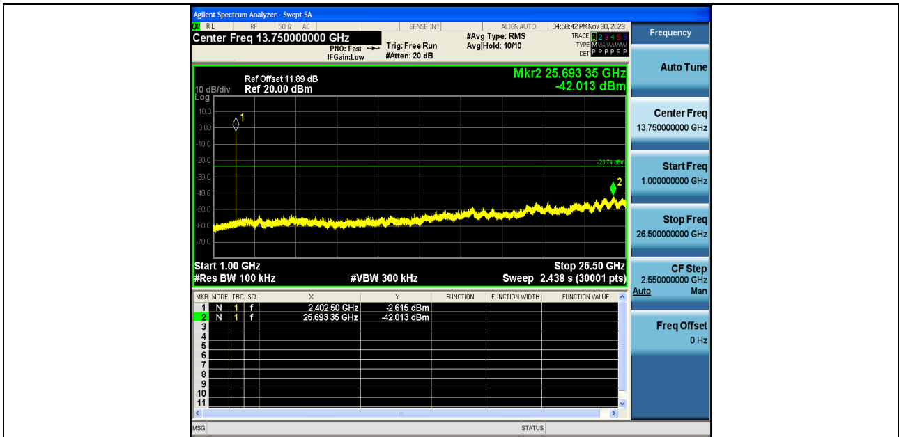
BLE_1M-Ant1-2402-1000~26500-PASS
