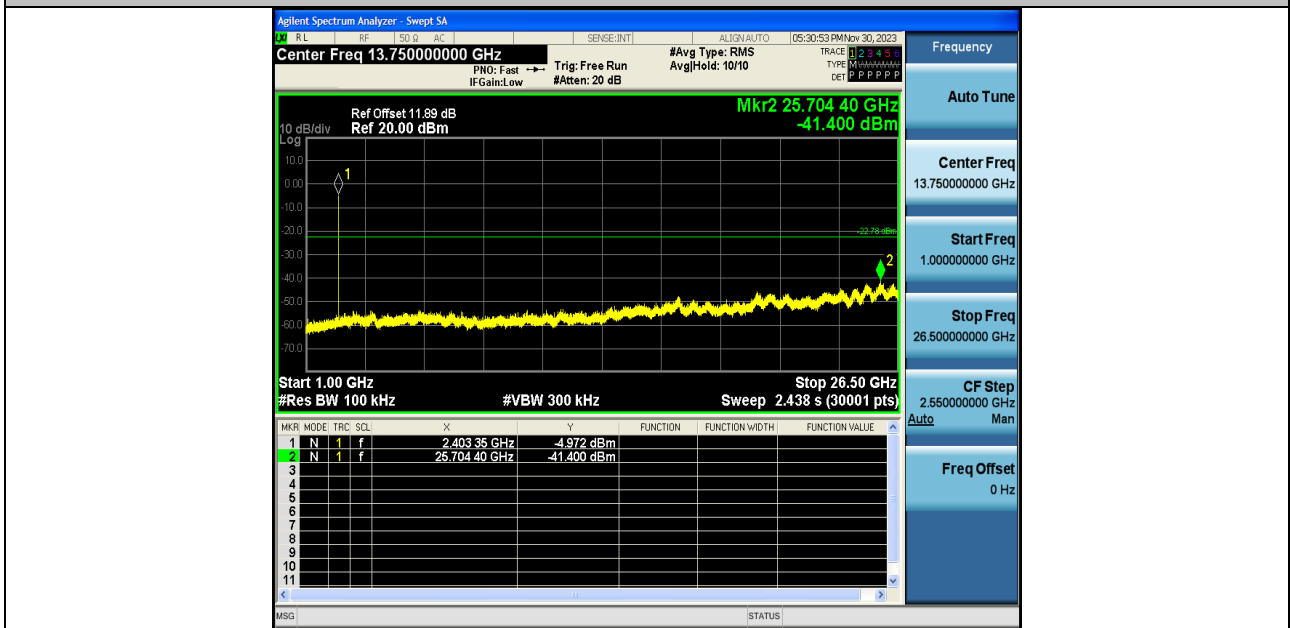
BLE_2M-Ant1-2404-1000~26500-PASS
