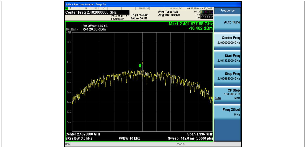
BLE_1M-Ant1-2402-PASS
