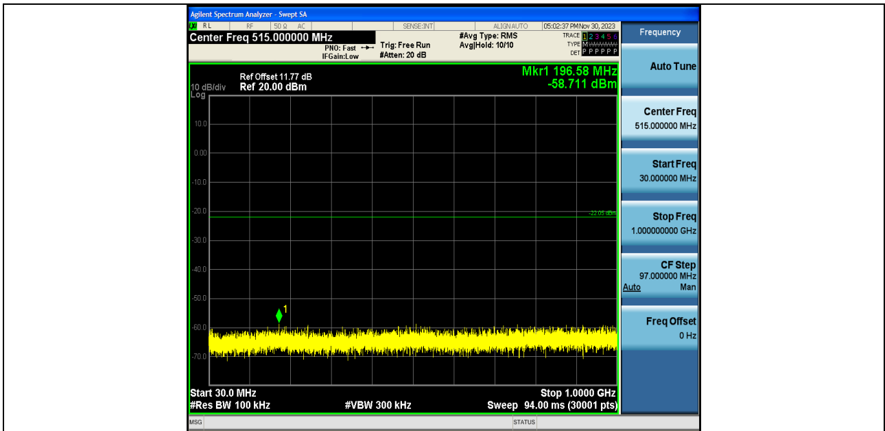
BLE_1M-Ant1-2440-30~1000-PASS
