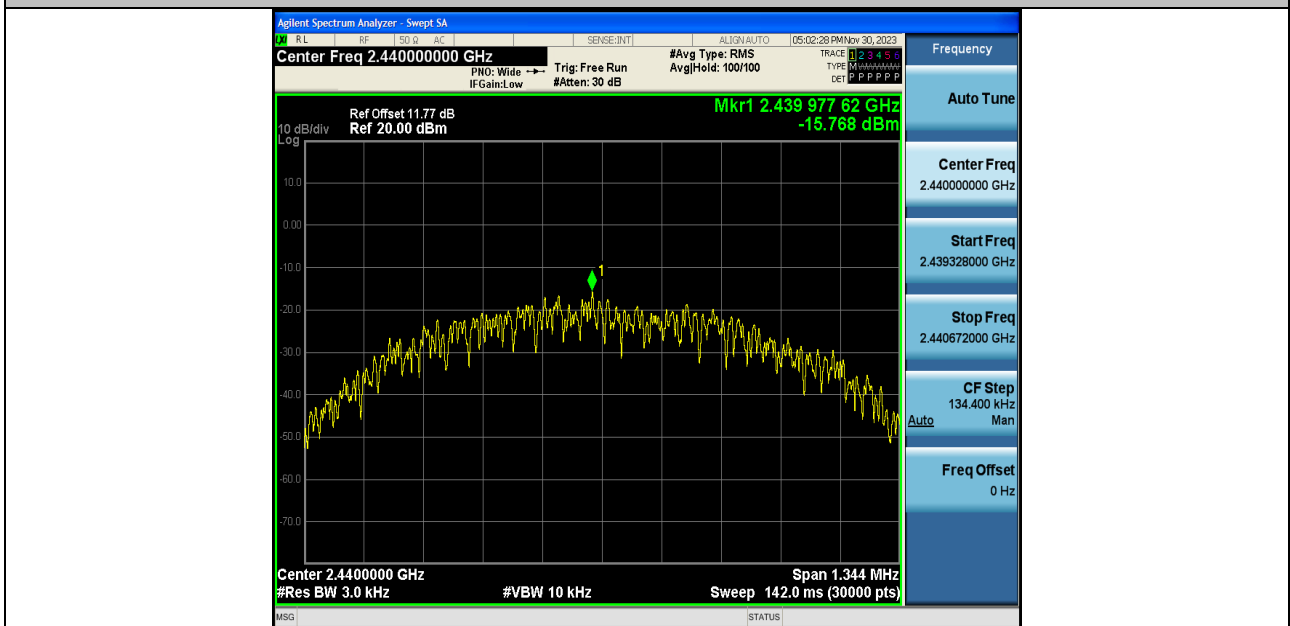
BLE_1M-Ant1-2440-PASS
