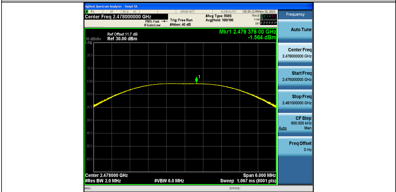
BLE_2M-Ant1-2478-PASS
