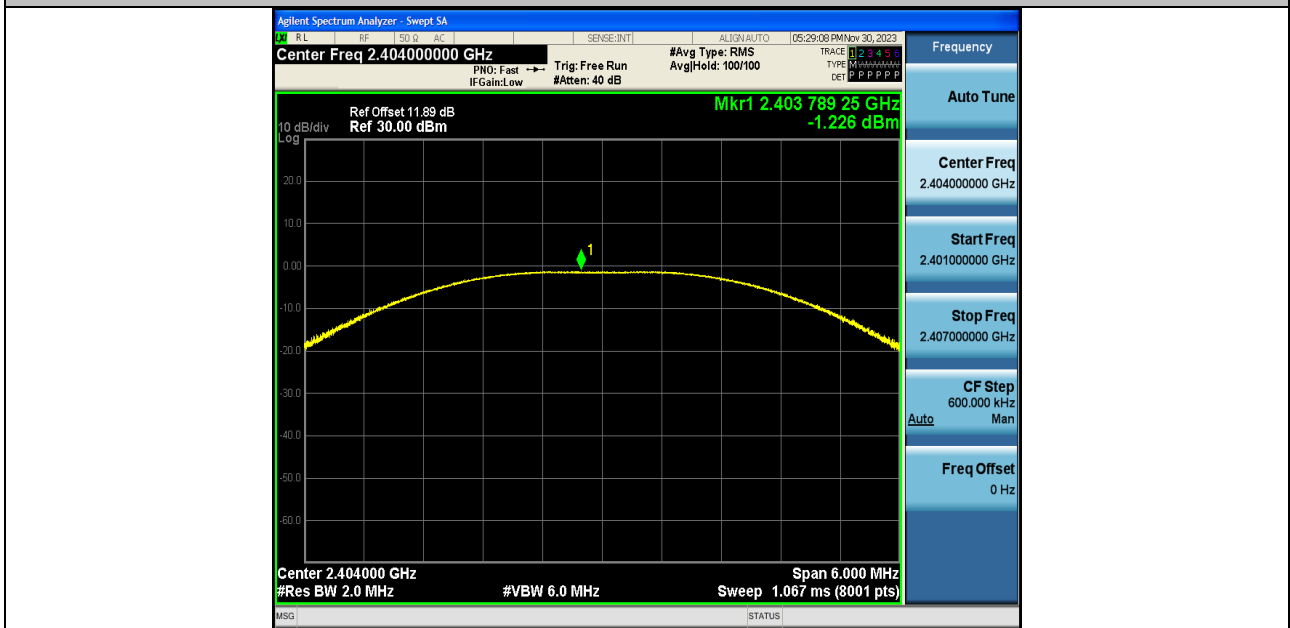
BLE_2M-Ant1-2404-PASS
