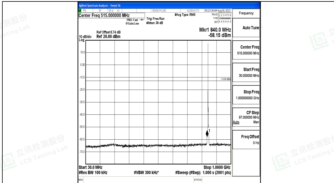
Band26_3MHz_QPSK_27025_1RB#0_30~1000_30~1000
