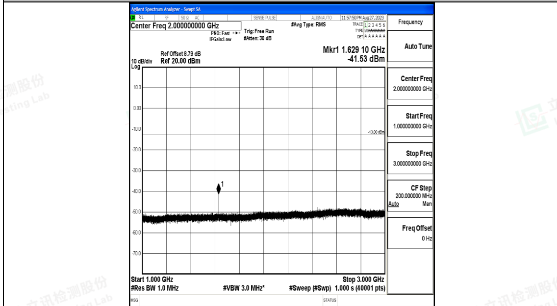
Band26_10MHz_QPSK_26740_1RB#0_1000~3000_1000~3000
