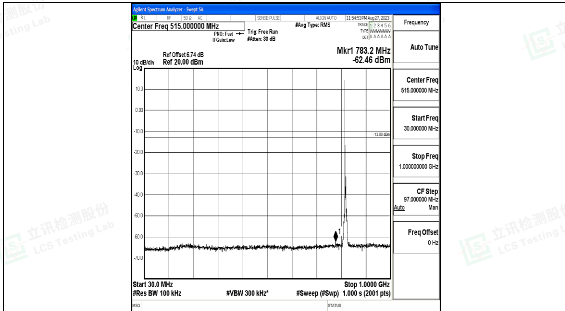
Band26_5MHz_QPSK_26765_1RB#0_30~1000_30~1000
