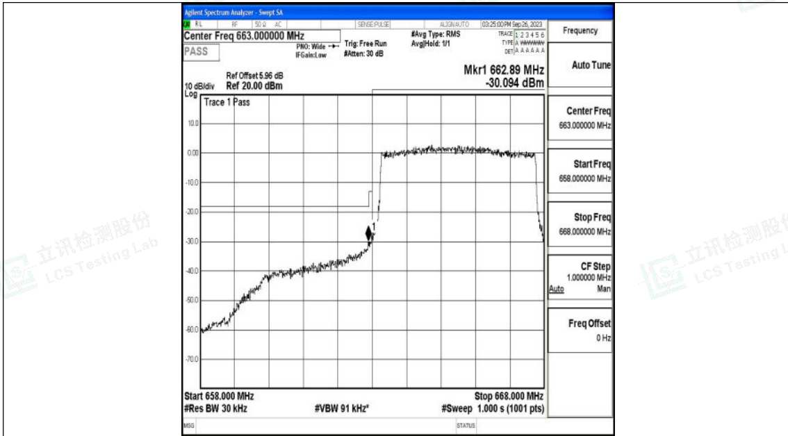
Band71_5MHz_QPSK_133147_25RB#0
