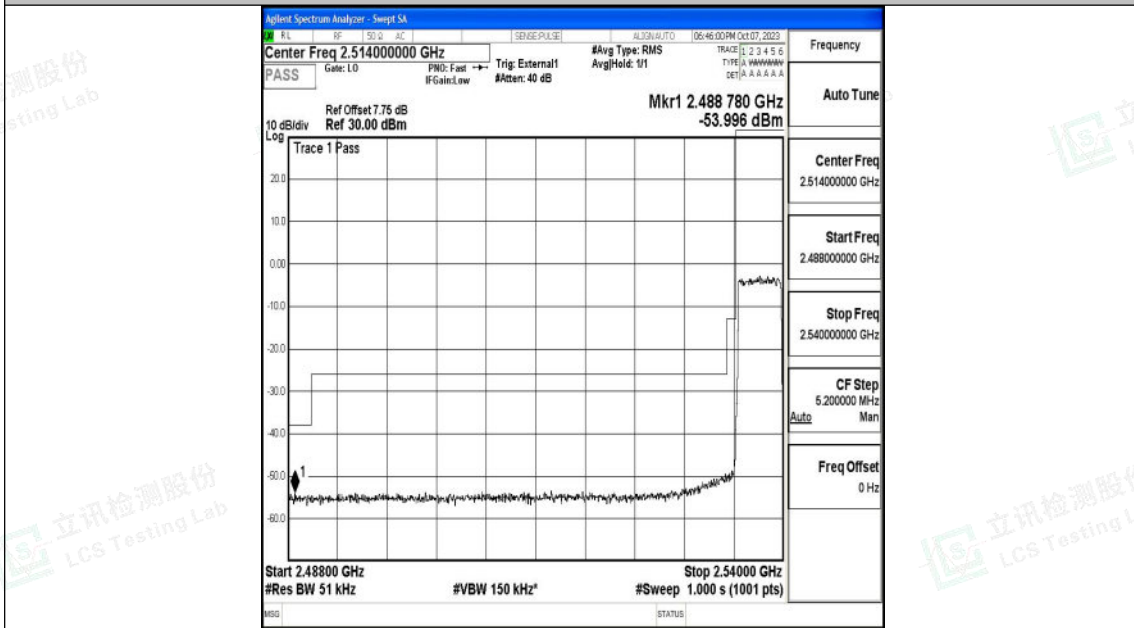
Band41_5MHz_16QAM_40065_25RB#0
