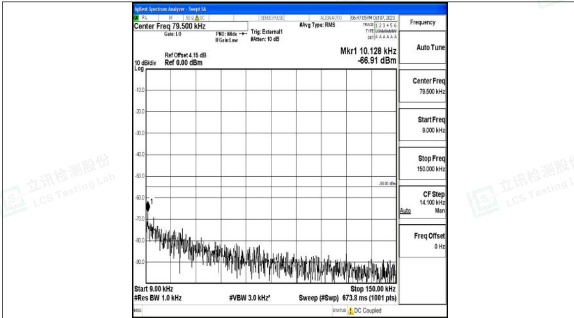
Band41_5MHz_QPSK_40065_1RB#0_0.009~0.15_0.009~0.15
