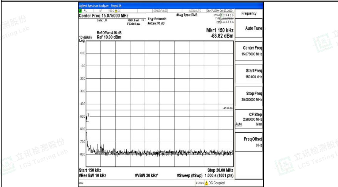
Band41_5MHz_QPSK_40065_1RB#0_0.15~30_0.15~30
