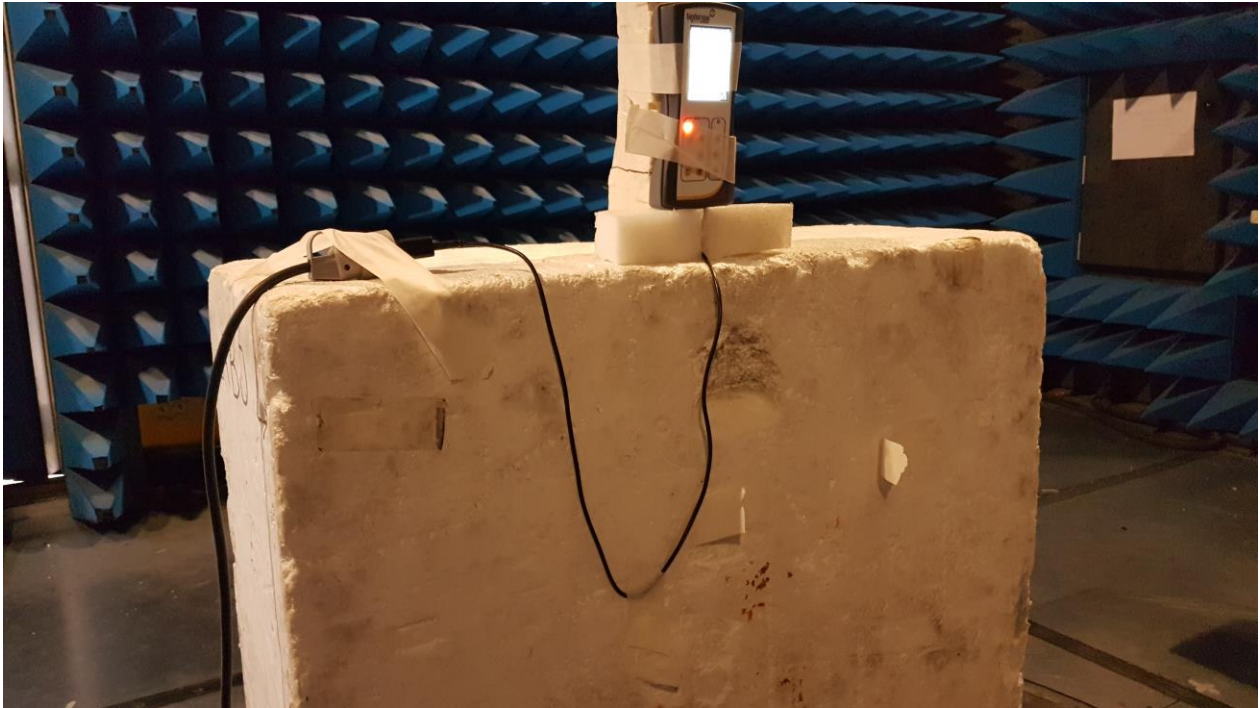
Anechoic chamber
