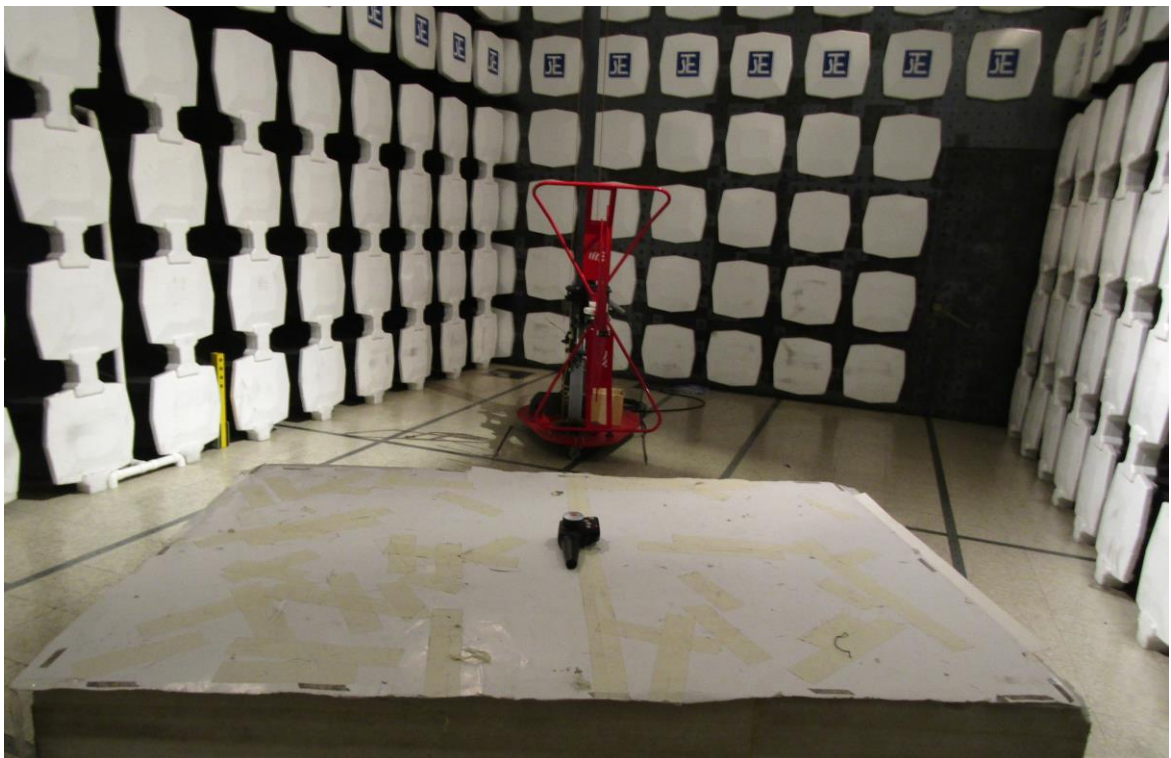
Measurement of Radiated Emission Test Set Up (30MHz to 1000MHz)
