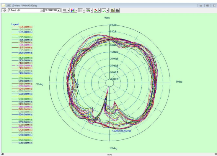
2.4GWIFI&Bluetooth&5G WIFI Phi=90deg
