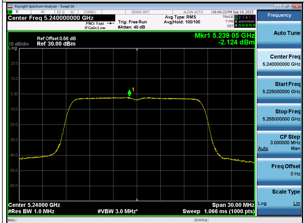
Test_Graph_802.11a_ANT2_5240_6Mbps_PSD
