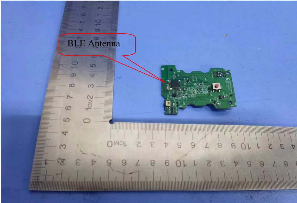
Photo 18 Appearance of PCB
