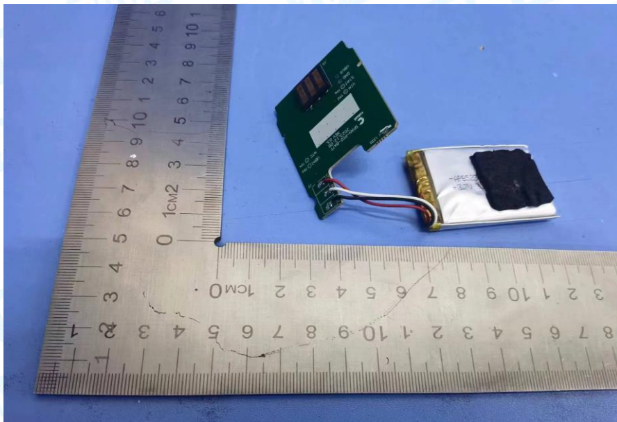
Photo 14 Appearance of PCB & Battery
