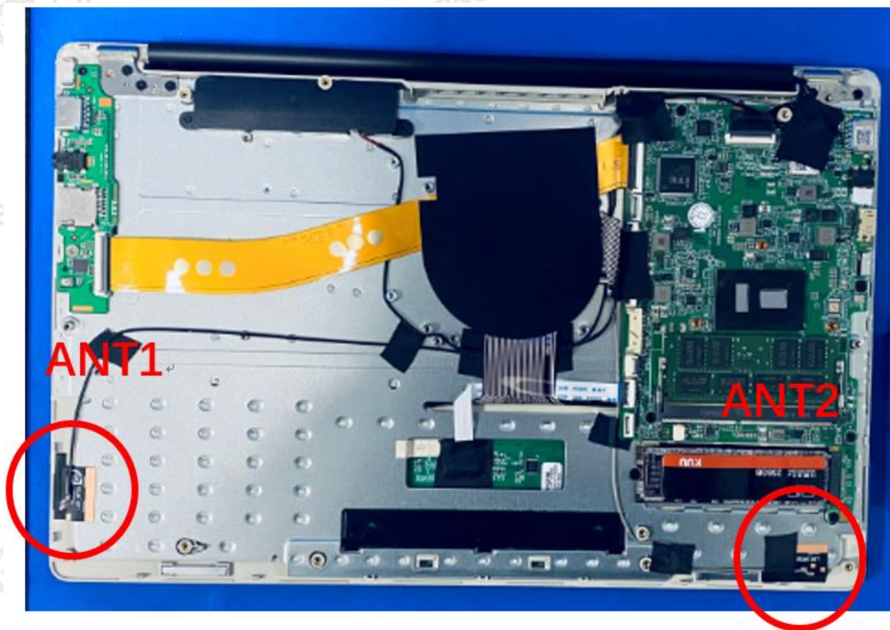
REAR VIEW
