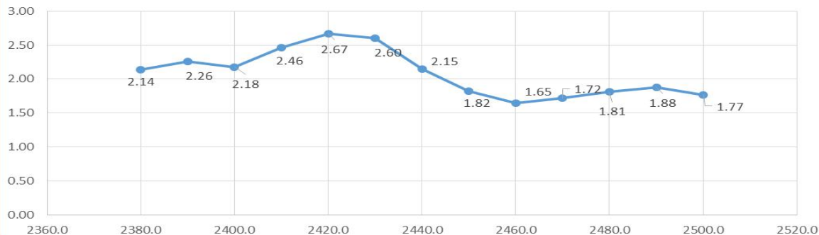
PeakGain (dBi)
