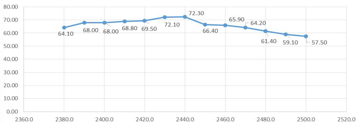
Efficiency (%)
